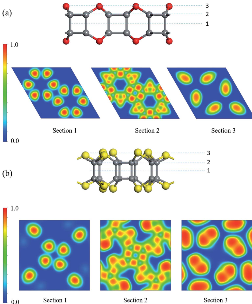
Fig. 3 ELF of (a) C 24 O 12 and (b) C 16 S 16 .
