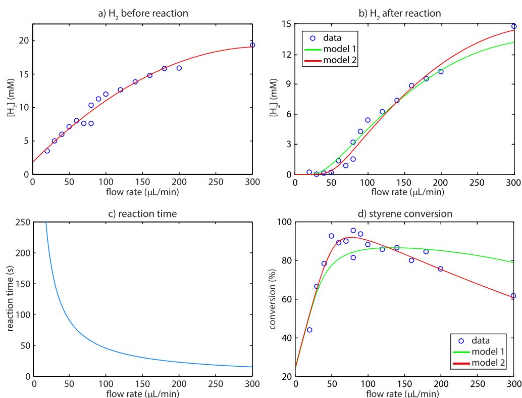
Figure 3. Hydrogenation of styrene: (a) concentration of hydrogen before the reaction and (b) after the reaction. (c) Calculated reaction times. (d) Styrene conversion including the fitted trends based on two models (see text).
