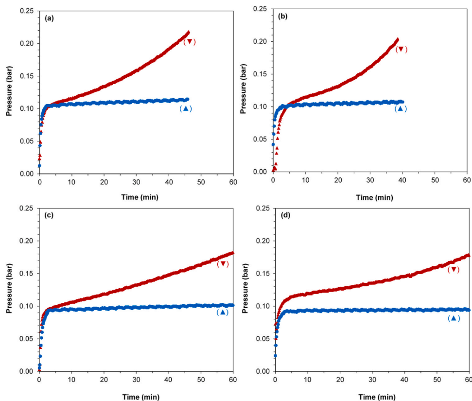
Fig. 7. Filtration at constant flux of 100 \text{ L/m}^2/\text{h} through 100 \text{ kDa} filter of the ( \blacktriangledown ) synthetic concentrate of 85% recovery (with phosphate) in the presence of 33.3 \text{ mg/L} of a) AS-D, b) AS-E, c) AS-G, and d) AS-H, and ( \blacktriangle ) synthetic concentrate of 85% (without phosphate) in the presence of 33.3 \text{ mg/L} of a) AS-D, b) AS-E, c) AS-G, and d) AS-H.
