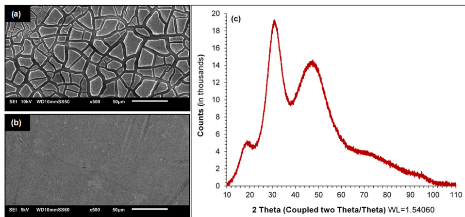
Fig. 4. a) SEM image (500× magnification) of the 0.45 μm filter after filtering the synthetic concentrate of 85% recovery, b) SEM image (500× magnification) of the 100 kDa filter after filtering the synthetic concentrate of 80% recovery, and c) XRD analysis of the retained deposits on the 0.45 μm filter after filtering the synthetic concentrate of 85% recovery.
