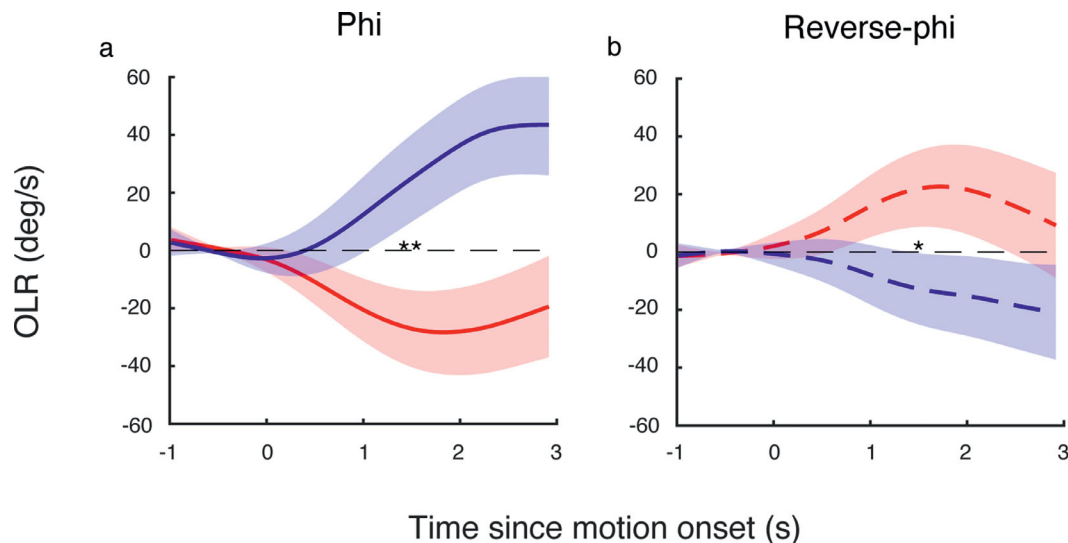
Figure 2. Comparison of OLR to phi and reverse-phi stimuli. (a) The mean opto-locomotor reflex over time for one mouse showing a typical OLR to rightward (red solid line) or leftward (blue solid line) phi stimuli. (b) Mean OLR for the same mouse to rightward (red dashed line) or leftward (blue dashed line) reverse-phi stimuli. The temporal interval in this example was 67 ms. Shaded bounds represent the SEM , asterisks indicate significant differences among OLRs (one-sided, two-sample t -test; * p < 0.05 , ** p < 0.01 ).
