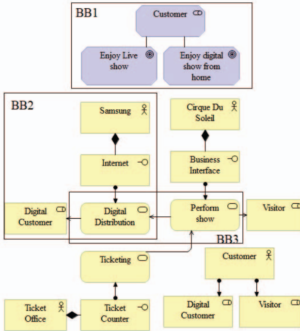
Fig. 8. Resulting ArchiMate model
