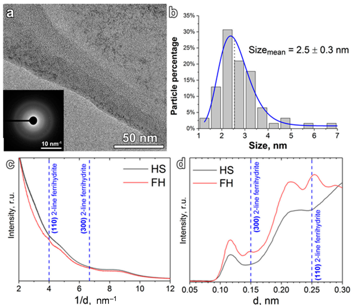
Figure 1. (a) TEM image of the synthesized ferrihydrate (FH) nanoparticles and the corresponding electron diffraction image (inset); (b) size distribution of nanoparticles in FH nanoparticles as revealed by TEM (log-normal fitting was used); (c) normalized electron diffraction integrals for the FH nanofertilizer and raw potassium humate (HS) (d is an interplane lattice spacing); (d) normalized background-subtracted electron diffraction of FH nanoparticles and raw potassium humate, replotted in d-space. Positions of the 2-line ferrihydrate reflections and lattice indexes assignments are given according to [60].
