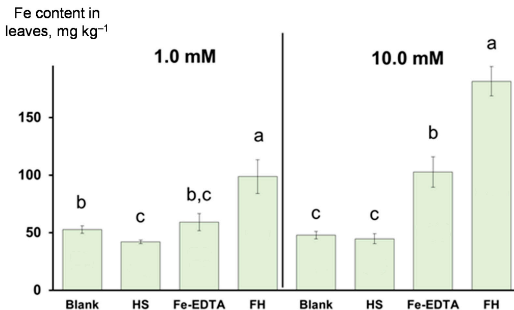
Figure 3. Iron content in the wheat leaves after foliar application of the iron-sources: ferrihydrate (FH) and ferric ammonium salt of ethylenediaminetetraacetic acid (Fe-EDTA), and control solutions: triple-distilled water (blank) and potassium humate (HS). The iron concentrations in the fertilizer sprays were 1.0 mM (left panel) and 10.0 mM (right panel). All treatments, except for the blank, contained urea adjuvant (0.2% wt.). The bars represent the standard deviation ( n = 4 ). The columns marked with different letters are significantly different at p < 0.05 according to the least significant difference (LSD) test.
