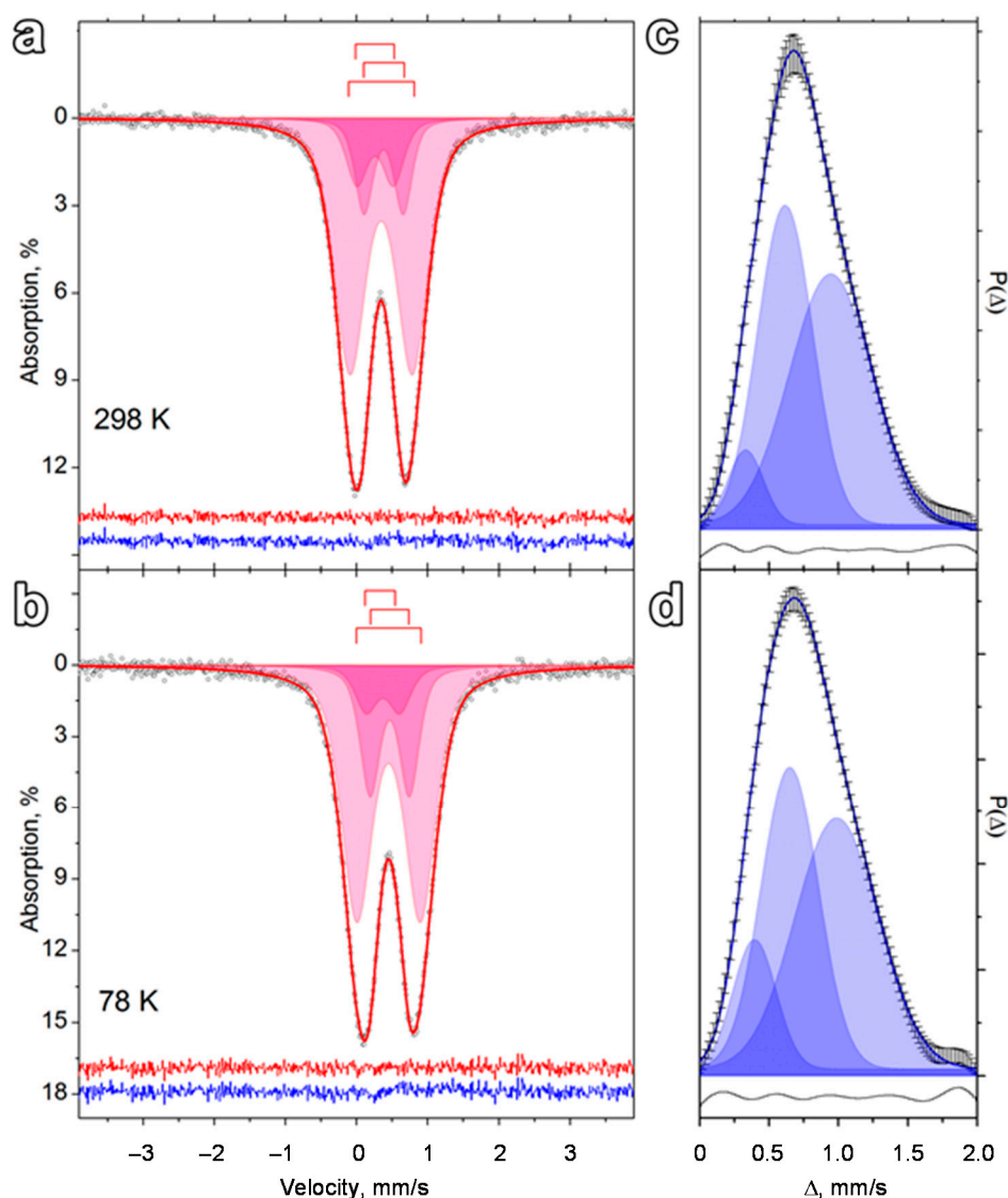
Figure 2. Mössbauer spectra at different temperatures of the ferrihydrite (FH) sample without urea treatment, models for their description (a,b), and the corresponding quadrupole splitting probability distribution functions (c,d).
