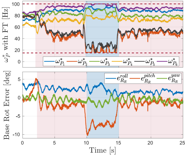
Fig. 3. Propellers commanded angular rates and base rotation error during pushing with disturbance. when the disturbance is applied, the propellers saturate. The robot error along the pitch direction increases to keep small the error of higher priority tasks, such as the contact force one.
