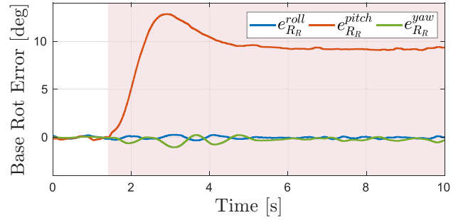
Fig. 10. Base rotation error while performing force control task in simulation. Due to the system's underactuation, the robot needs to tilt in order to achieve the required contact force.
