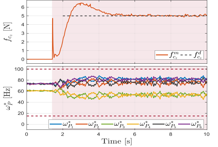
Fig. 9. Normal force during contact (top plot) and propellers velocities (bottom plot) in simulation. The robot can successfully achieve force control tasks despite the underactuation.
