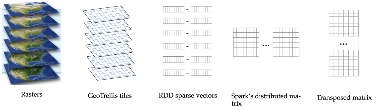
Fig. 2. From GeoTIFFs to a Spark's distributed matrix.
