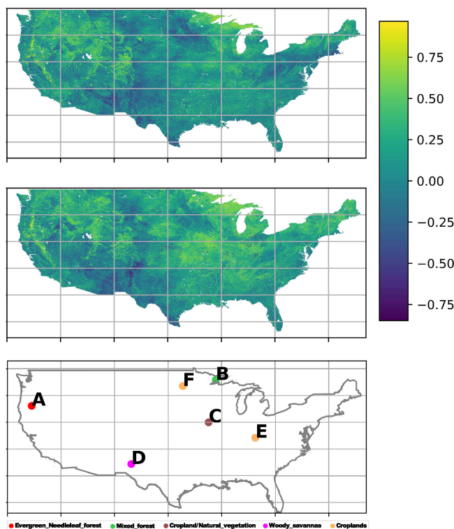
Fig. 6. Correlation between the Leaf index and SOS [Top], between the Bloom index and SOS [Middle], and sampled grid cells for further analysis [Bottom].
