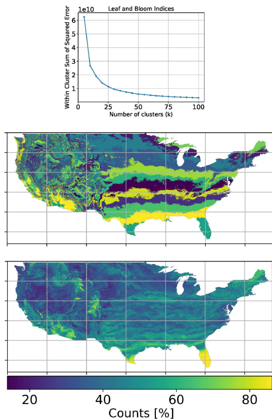
Fig. 5. Within-cluster sum of squared Errors versus the number of clusters for Leaf and Bloom [Top]. Clustering maps for mode of Leaf and Bloom clustering [Middle]. Percentage of counts for each mode [Bottom].
