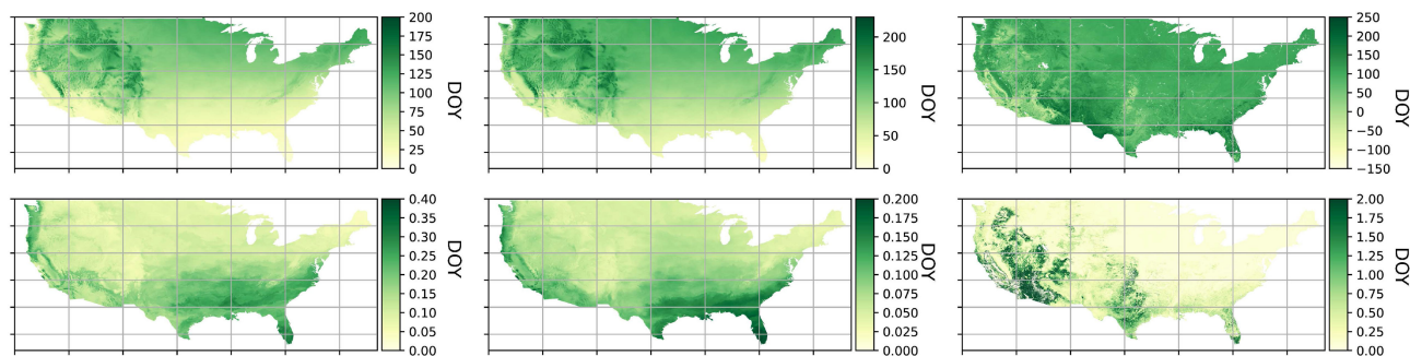
Fig. 3. Top: Average of Leaf and Bloom indices and AVHRR Start of Season (SOS) maps of conterminous US from 1989 to 2014. Bottom: The coefficient of variation of Leaf and Bloom indices and AVHRR SOS maps of conterminous US from 1989 to 2014.
