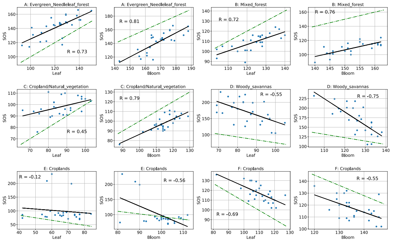
Fig. 7. Crossplots between the Leaf/Bloom index and SOS for the grid cells shown in Fig. 6. The black lines show the corresponding linear fits, the dashed green lines indicate the 1:1 line, the R values are the Pearson correlation coefficients and the titles list the MODIS-extracted land cover types.
