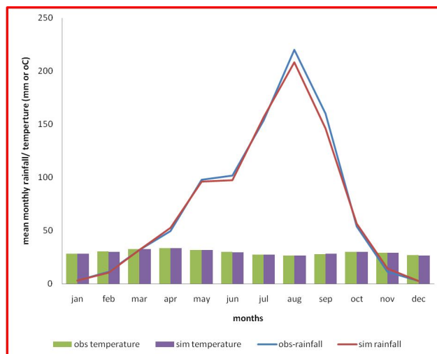
Fig. 3: Comparison of observed/baseline and simulated mean monthly rainfall and temperature for Volta basin.
