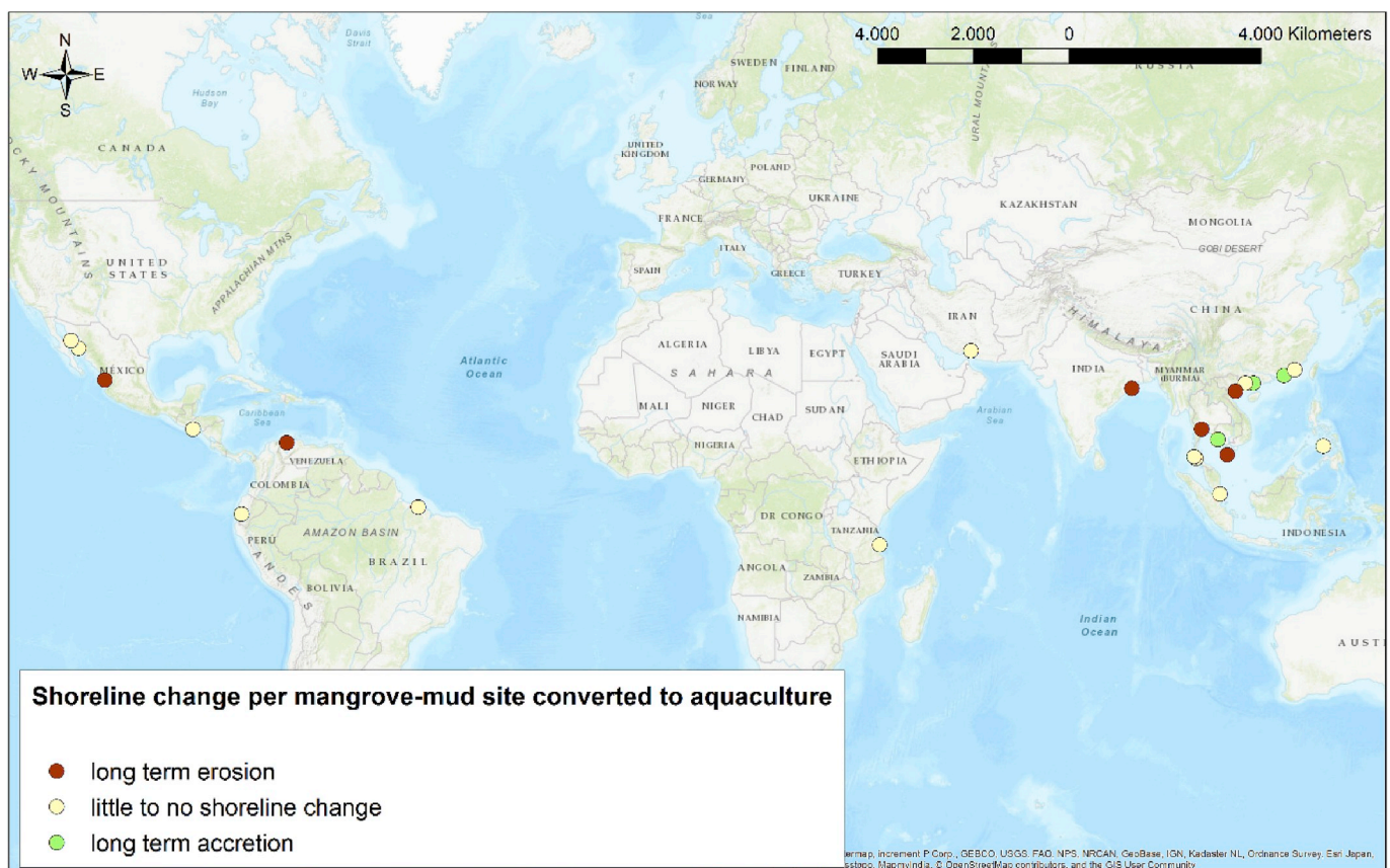
Fig. 1. Long term shore line changes from 1984 until 2016 as reported by Luijendijk et al. (2018) averaged per aquaculture coast. Aquaculture coasts displayed are sites designated by RAMSAR as internationally important wetlands, distinguished by mangroves and mudflats that have been (partly) converted to aquaculture (RAMSAR, 2018).
