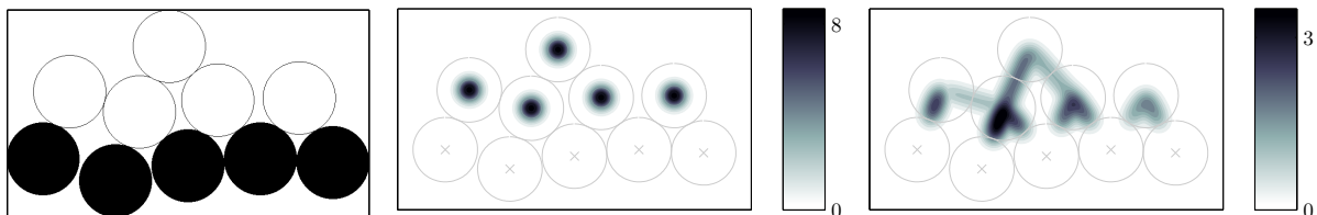
Figure 8: Snapshot of the final state of the FiveParticles simulation (left). Coarse-graining is applied to obtain the bulk density \rho (centre) and pressure p (right).
