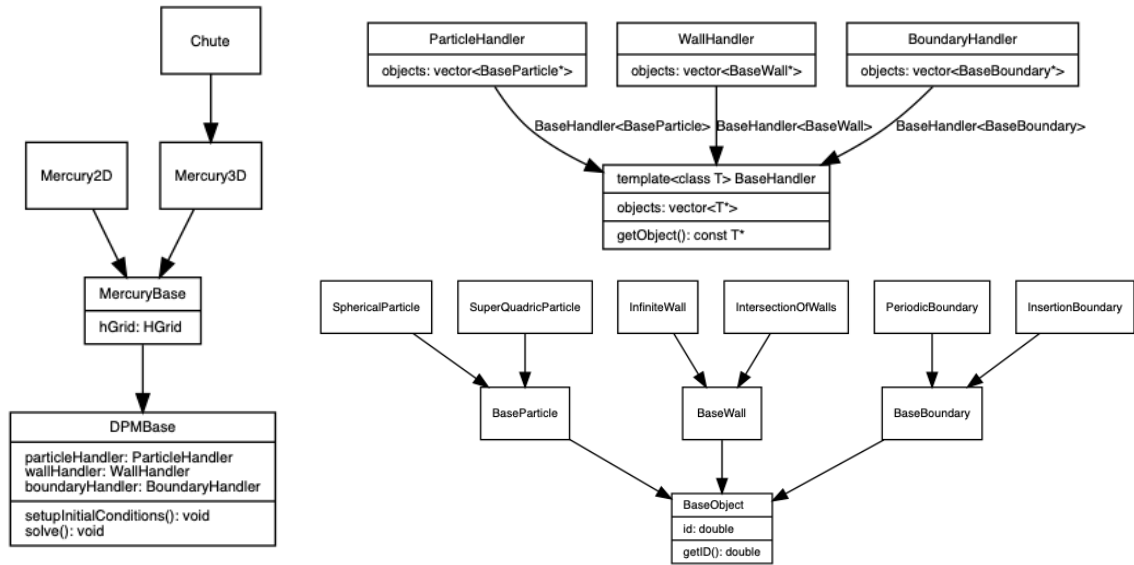
Figure 5: Basic class structure of MercuryDPM , showing the inheritance and encapsulation strategy. Handlers for contact laws, interactions, coarse-graining, and MPI decomposition are not shown, and only a select number of particle, wall, and boundary types are shown.
