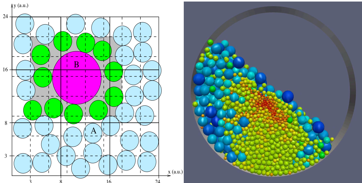
Figure 6: (left) A two-level grid for the special case of a bi-disperse system. The first level grid is plotted with dashed lines while the second level is plotted with solid lines.
