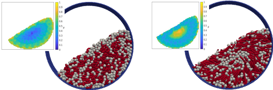
Figure 3: Mixtures of spheres and ellipsoidal particles in a rotating drum, screenshots and coarse-grained solid volume fraction of spheres. ( left ) ellipsoids of aspect ratio 2, ( right ) ellipsoids of aspect ratio 4.
