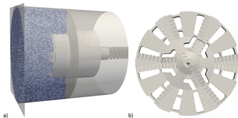
Figure 2 (a) EPB and soil simulated with MercuryDPM ; (b) Cutterhead created with triangulated walls [10]
