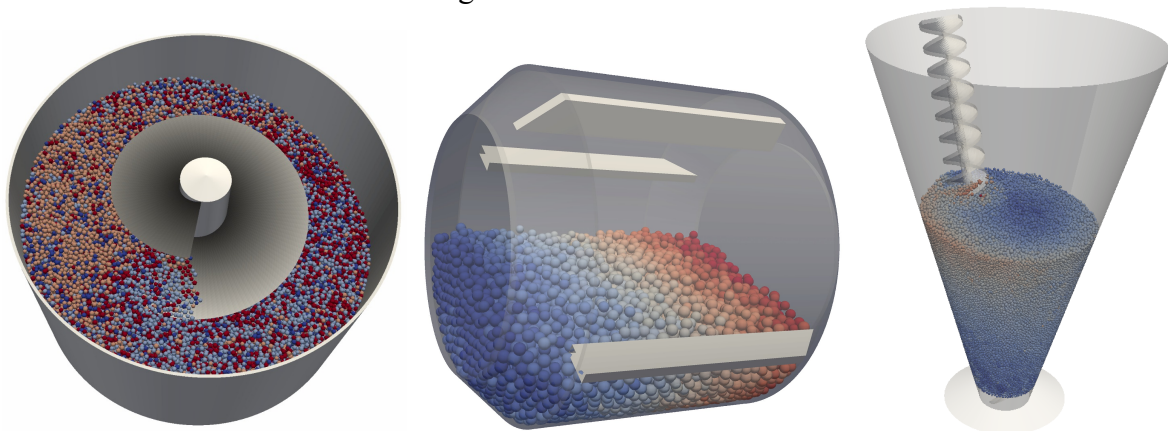
Figure 1 Industrial mixers simulated in MercuryDPM with curved geometric features (no triangulation). Left-to-right: Auger mixer, rotating drum, and Nauta mixer.
