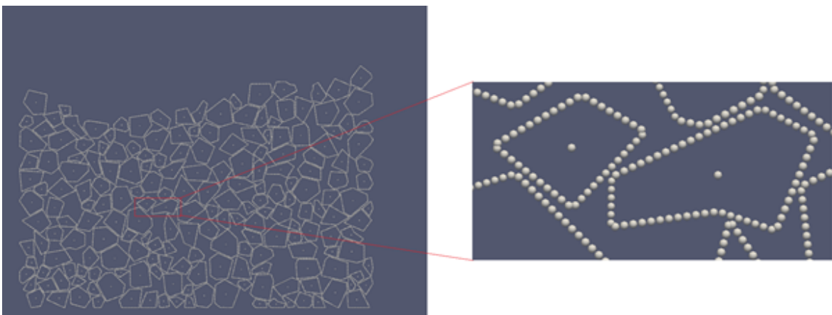
Figure 4: Multispheres reproducing the shape of ballast particles in a simulated compression test.
