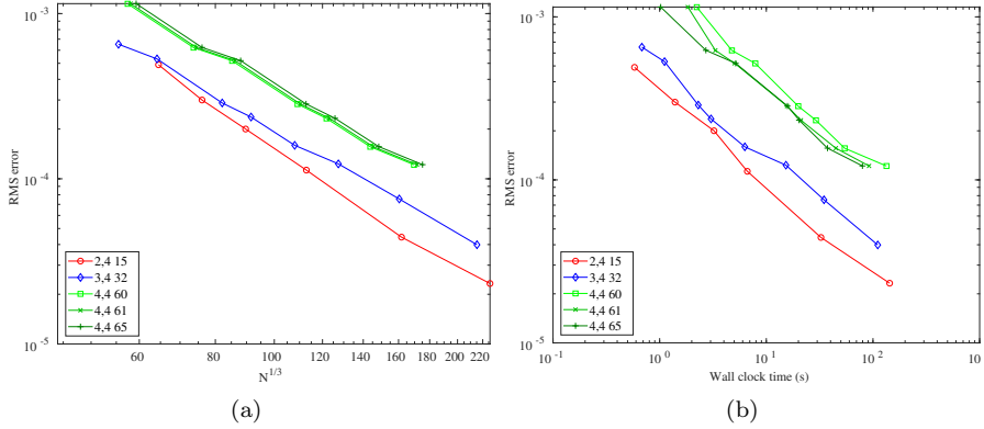
FIG. 4. Same as Figure 3, but using exact integration to evaluate the stiffness matrix and using a piecewise constant approximation of the mass density \rho . All methods only converge with second order due to the parameter approximation and higher-degree methods only result in more degrees of freedom and computation time.
