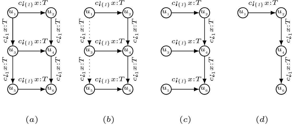
Figure 5. EVRSP from G_1 \square G_3 (a), two stages of G_1 \boxtimes G_3 (b,c), to G_1 \boxdot G_3 (d).
