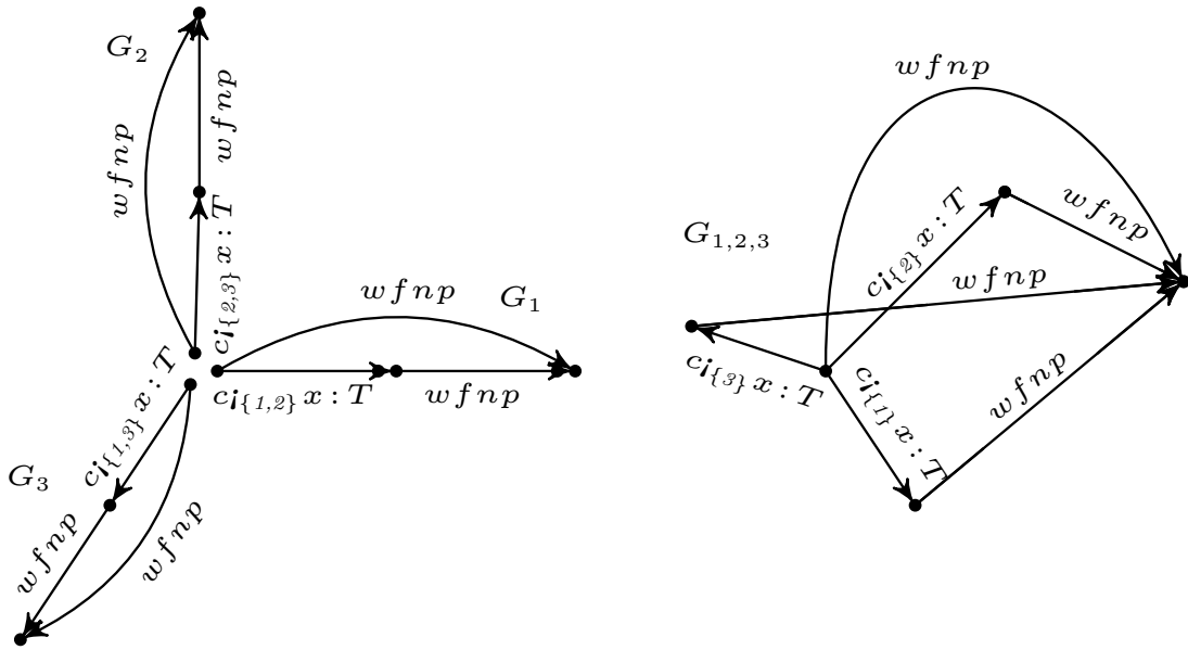
Figure 3. Graphs G_1, G_2, G_3 , and G_{1,2,3} = \bigboxtimes_{i=1}^3 G_i representing processes P_1, P_2, P_3 , and their parallel composition (P_{1_{x_1}} \uparrow_{x_2} P_2)_{x_1 \cup x_2} \uparrow_{x_3} P_3 of Listing 2.
