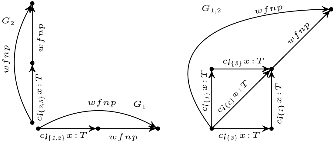
Figure 2. Graphs G_1, G_2 , and G_{1,2} = \overset{\circ}{\boxtimes}_{i=1}^2 G_i representing processes P_1 and P_2 , and their parallel composition ( P_{1 \times_1} \uparrow_{\times_2} P_2 ) of Listing 2.
