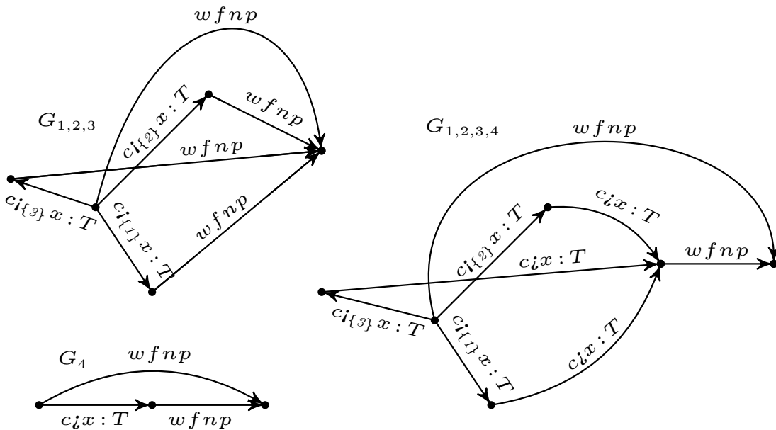
Figure 4. Graphs G_{1,2,3}, G_4 , and G_{1,2,3,4} = \bigboxtimes_{i=1}^4 G_i representing processes (P_{1_{x_1}} \uparrow_{x_2} P_2)_{x_1 \cup x_2} \uparrow_{x_3} P_3, P_4 , and their parallel composition ((P_{1_{x_1}} \uparrow_{x_2} P_2)_{x_1 \cup x_2} \uparrow_{x_3} P_3)_{x_1 \cup x_2 \cup x_3} \uparrow_{x_4} P_4 of Listing 2.
