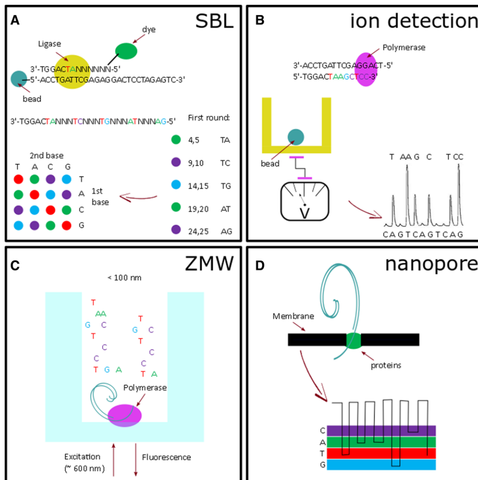
Figure 3. Overview of several DNA sequencing techniques with the principle of (A) sequencing by ligation (SBL, e.g. SOLiD®), (B) ion detection (e.g. Ion Torrent™), (C) zero-mode waveguides (ZMWs, e.g. PacBio®) and (D) nanopores (e.g. Oxford Nanopore).
