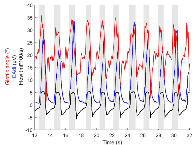
Fig. 3. Example of EAdi, flow and angle of the glottis of 1 subject during 1 setting. Grey areas represent inspiration based on EAdi, from > 2 μV to 80% of peak EAdi.
