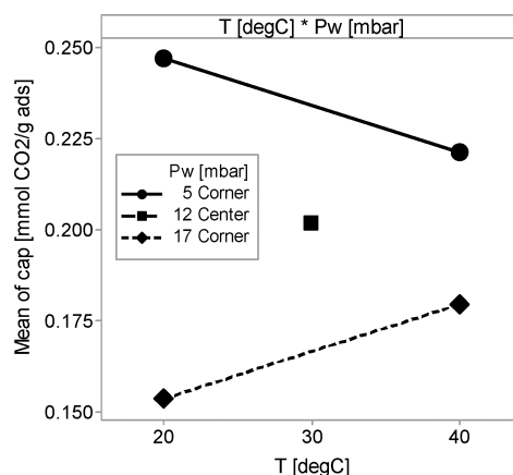
Figure 10. T – P_w interaction plot for the capture capacity data.
