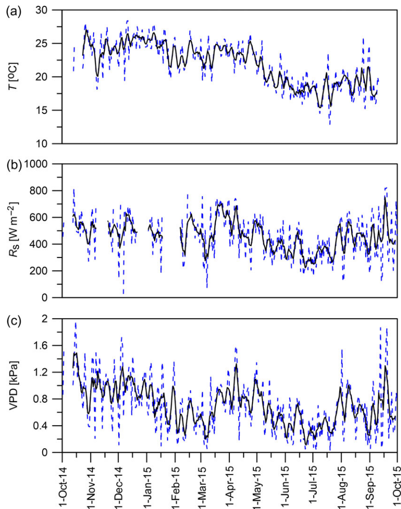
Figure 1. Daily averages (dashed lines) and 5-day moving averages (solid lines) of (a) above-canopy air temperature ( T , ^{\circ}\text{C} ), (b) incoming short-wave radiation ( R_s , \text{W m}^{-2} ) and (c) vapour pressure deficit (VPD, \text{kPa} ) for the investigated young secondary forest site near Andasibe between 1 October 2014 and 30 September 2015.
