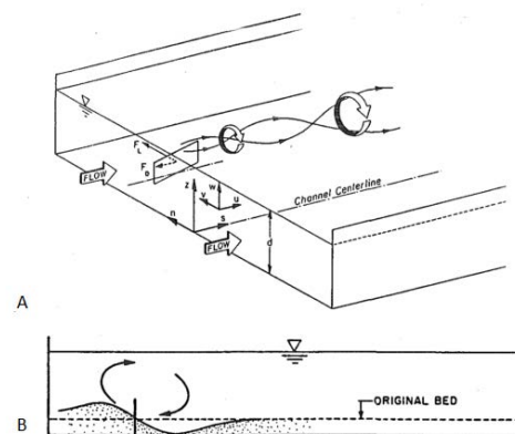
Figure 1: Vane-induced circulation (A); resulting bed-morphology (B) (Odgaard and Wang, 1991)
