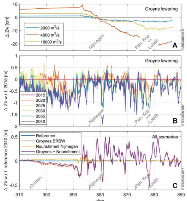
Figure 1. Hydro-morphologic effects of groyne lowering and two nourishment scenarios plotted along the river (rkm is kilometres along the river axis). A) illustrates the initial change in water level after lowering of all groynes along the Boven-Rijn and Boven-Waal (BRBW), as computed by Waqua. B) shows change in bed level elevation (w.r.t. the situation in 2015) caused by the groyne lowering along the BRBW (Delft3D). C) shows the difference between the bed level elevation for each scenario and the reference situation in 2040 (Delft3D).
