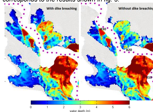
Figure 3: Water depth of the 2D part on 29 March at 00:00 (left: with dike breaching and right: without). Purple dots are river kilometres (805-840).
