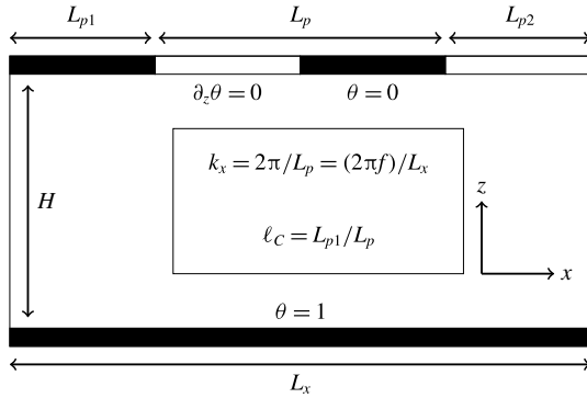
FIGURE 1. The 2D y-cut of the geometry. The domain has dimensions L_x \times L_y \times H . The bottom plate, at \hat{z} = 0 , has \theta = 1 . The top plate is divided into stripes of conducting ( \theta = 0 ) and insulating ( \partial_z \theta = 0 ) regions.
