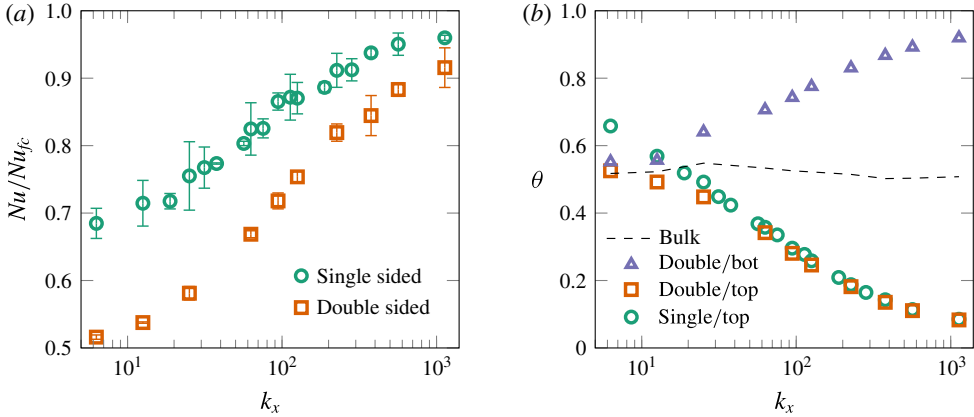
FIGURE 8. (Colour online) (a) Comparison of the normalized Nusselt number Nu/Nu_{fc} for the single- and double-sided cases with Ra = 10^8 , Pr = 1 and \ell_C = 0.5 . For the lowest k_x , we see that the system is about two-thirds and one-half of the fully conducting case for the single- and double-sided cases, respectively. (b) Average temperature above or below the insulating stripes for the single- and double-sided cases with Ra = 10^8 , Pr = 1 and \ell_C = 0.5 . The dashed line shows the average bulk temperature, calculated at mid-height for the double-sided system.
