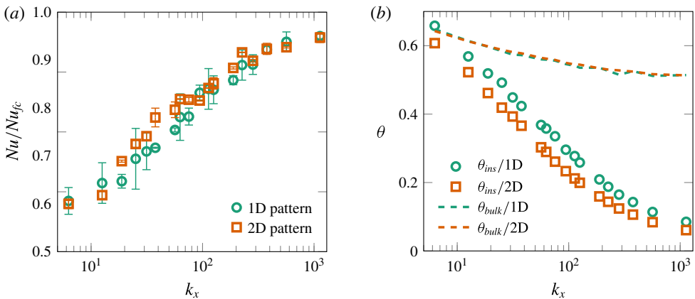
FIGURE 12. (Colour online) (a) Normalized Nusselt number Nu/Nu_c for 1D and 2D patterning versus k_x for Ra = 10^8 and Pr = 1 . The error bars show the statistical convergence error. (b) Average temperature \theta_{in} just below the insulating area and average bulk temperature \theta_{bu} , both as a function of k_x for the 1D and 2D patterning. The Ra and Pr values are the same as for panel (a).
