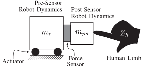
Fig. 3. Generic electromechanical system overview of an admittance controlled device. An actuator moves all mechanics (robot inertia m_r and some dissipation) placed before (i.e. ‘pre’) the force sensor. Behind the force sensor (i.e. ‘post’) there will be mechanics that generate force sensor measurements during motion ( m_{ps} ). These post sensor mechanics consequently interact with the human limb Z_h . The sensor is assumed to be infinitely stiff and its inertia is absorbed in m_{ps} .
