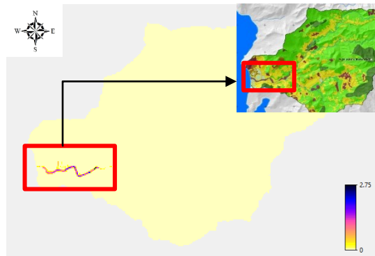
Figure 7. Flood depth of St. John's watershed (m) at 5 years return period
