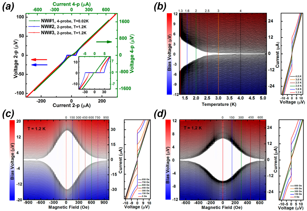
FIG. 3. Electric-transport characteristics for the Nb/Cu-nanowire/Nb junctions: (a) green, blue, and red lines are I(V) characteristics of the samples NW#1, NW#2, and NW#3, respectively; the inset is a zoom of I(V) plots. (b) Dependence of I(V) curves on the temperature for the sample NW#3. (c) and (d) I(V) dependencies as a function of perpendicular magnetic field H for the NW#2 and NW#3, respectively; the measurement temperature is T = 1.2 K. I(V) curves shown to the right of the panels (b), (c), (d) correspond to the sections of the 3D graphs at certain temperature or magnetic field values.
