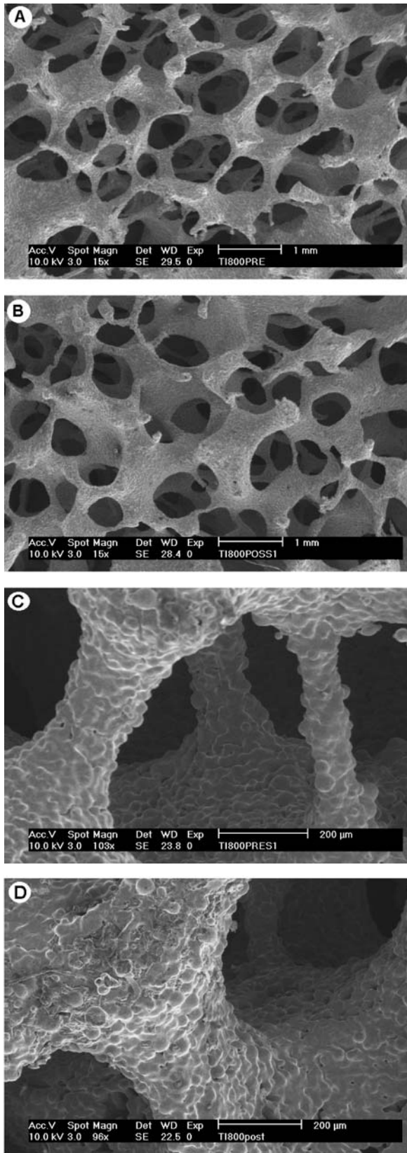
Figure 3 Macrostructure and microstructure of porous Ti6Al4V. (a) Macrostructure without any additional coating, (b) Macrostructure with one time coating, (c) Struts without any extra coating, (d) Struts with one time coating, (e) Cancellous bone. (Continued on next page.)
