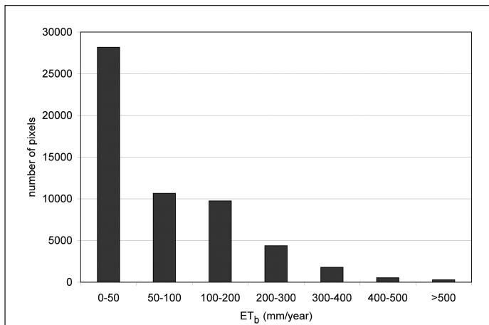
Figure 7. Yearly accumulated ET_b histogram in the region of Europe.
