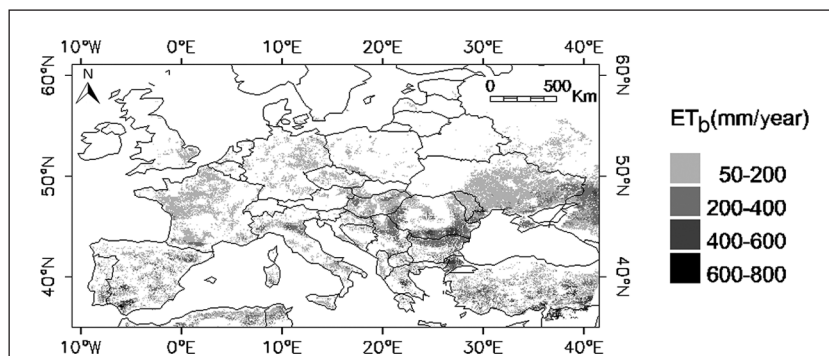
Figure 8. Yearly ET_b obtained with the proposed method in Europe during 2008 calculated in croplands according to the GlobCover map (irrigated and rainfed croplands, and mixed classes that include croplands).
