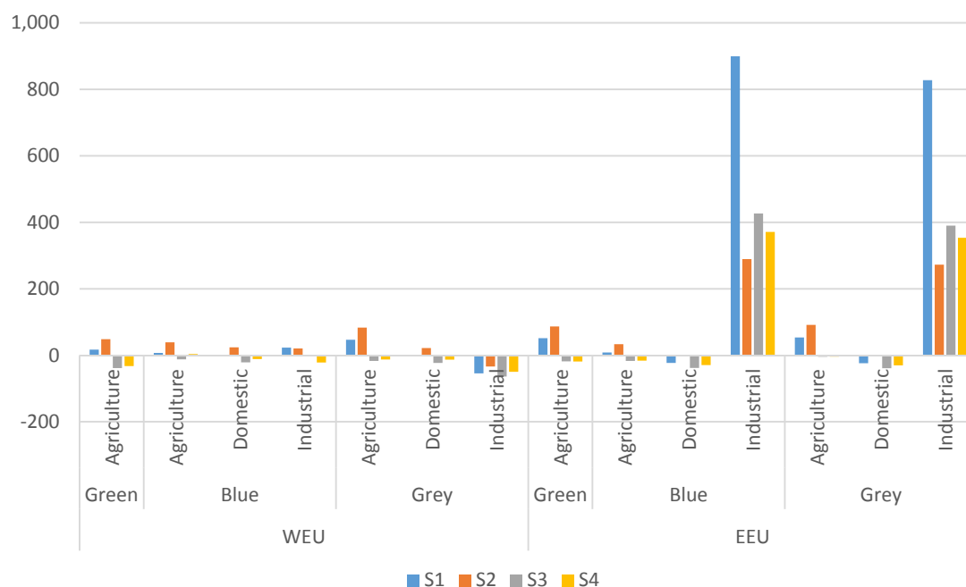
Figure 1. Percentage change in the WF of total production in WEU and EEU relative to 2000.
