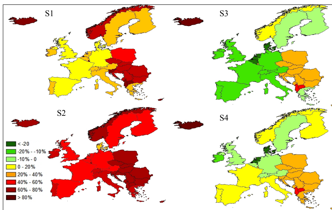
Figure 2. Percentage change of the WF of total production relative to 2000.
