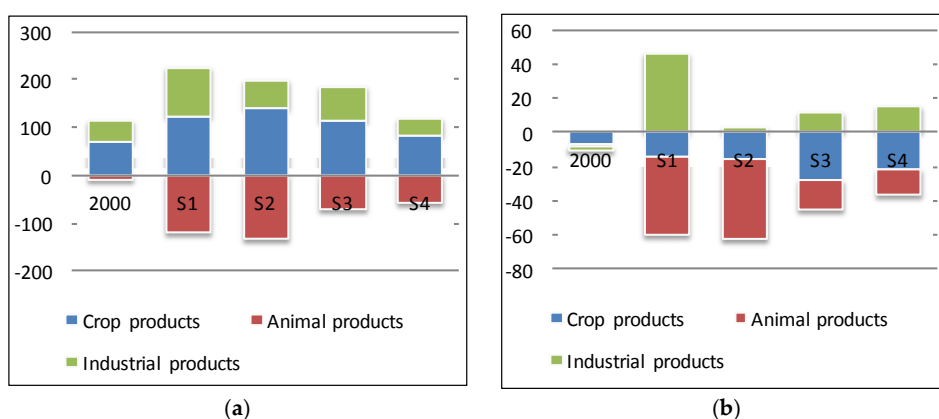
Figure 7. Net virtual water import by (a) Western Europe (WEU) and (b) Eastern Europe (EEU) (billion m 3 /year), specified by commodity group. Positive values represent net virtual water import; negative values represent net virtual water export.
