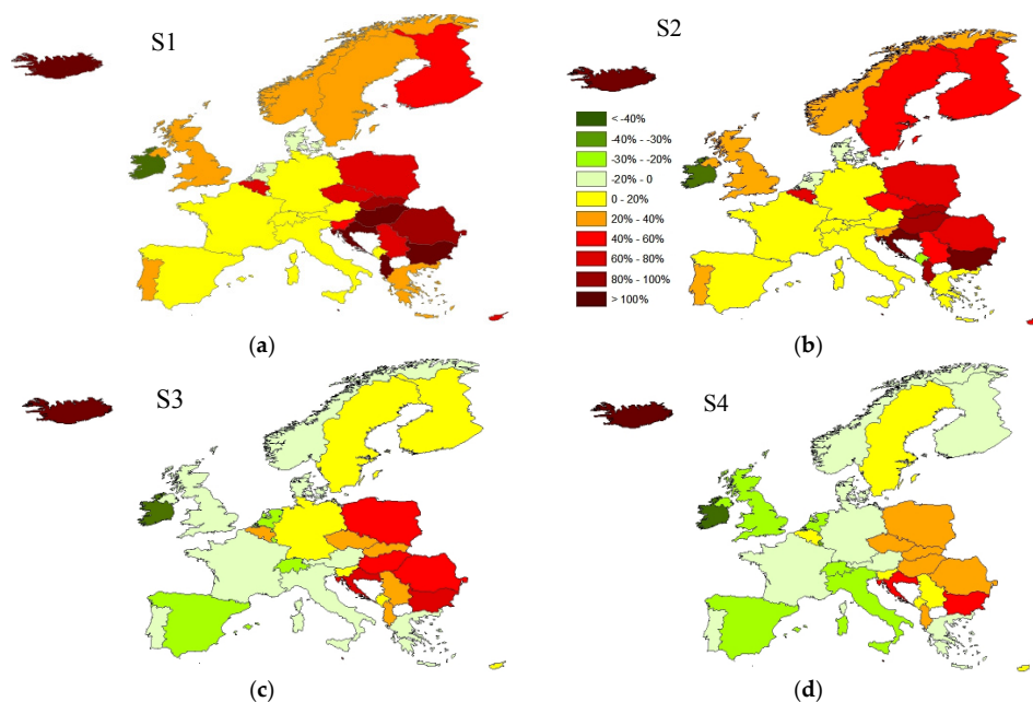
Figure 12. Percentage change in the water footprint (WF) of consumption per capita relative to 2000 in scenarios (a) S1, (b) S2, (c) S3 and (d) S4.
