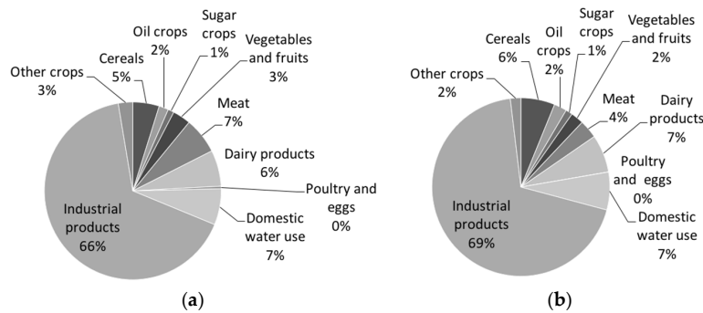
Figure 11. The composition of the grey water footprint (WF) of European consumption by commodity in scenarios (a) S1/S2 and (b) S3/S4.
