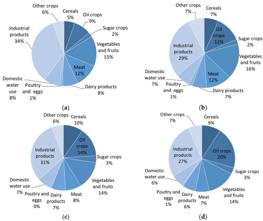
Figure 10. The composition of the blue water footprint (WF) of European consumption by commodity in scenarios (a) S1, (b) S2, (c) S3 and (d) S4.
