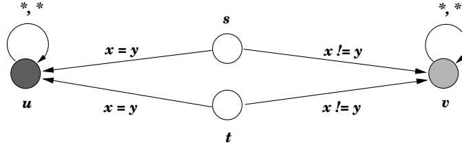
Figure 5: s \sqsubseteq_1^\Gamma t but s \not\preceq_1 t and s \cong_1^\Gamma t but s \not\preceq_g t
