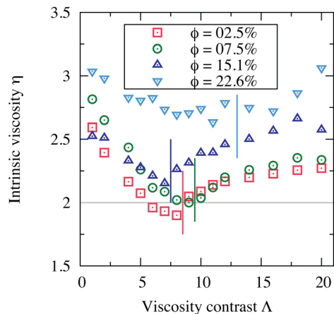
Fig. 6 The intrinsic viscosity \eta versus the viscosity contrast \Lambda of four suspensions with concentrations \phi = 2.5\% , 7.5\% , 15.1\% and 22.6\% . The vertical lines denote the minima of the curves. For every given value of \Lambda , a suspension becomes more and more viscous with increasing \phi . For the dense suspension ( \phi = 22.6\% ), the non-monotonic behavior of \eta with \Lambda is less pronounced. Furthermore, the viscosity contrast of the minimum of \eta does not vary in a monotonic way with \phi . Other parameters: Re = 0.5 , Ca = 10 , \Delta = 0.8 and \chi = 0.2 .
