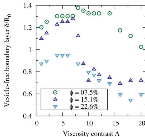
Fig. 7 The rescaled vesicle-free boundary layer \delta/R_0 versus the viscosity contrast \Lambda of three suspensions with concentrations \phi = 7.5\% , 15.1\% and 22.6\% . For all three concentrations, \delta/R_0 increases for low \Lambda and then decreases for high \Lambda . Its maximum coincides neither with the critical viscosity contrast of the tank-treading-to-tumbling transition nor with the minimum of the intrinsic viscosity. It does shift towards lower values of \Lambda with increasing \phi . Other parameters: Re = 0.5 , Ca = 10 , \Delta = 0.8 and \chi = 0.2 .
