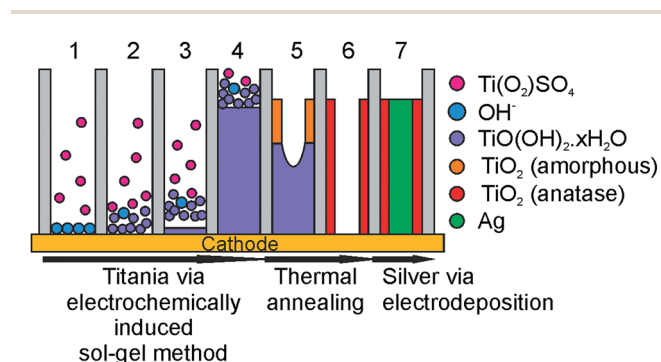
Fig. 1 Schematic overview of the preparation of coaxial \text{TiO}_2 -Ag nanowires using the electrochemically induced sol-gel method: formation of \text{OH}^- at the electrode (step 1, reaction (2)), reaction of \text{Ti}(\text{O}_2)\text{SO}_4 with \text{OH}^- to form \text{TiO}(\text{OH})_2 \cdot x\text{H}_2\text{O} and filling of the template (steps 2-4, reaction (3)), drying and thermal annealing of the titanium hydroxide gel to \text{TiO}_2 (steps 5-6, reaction (4)), and filling of the \text{TiO}_2 nanotubes with Ag (step 7).
