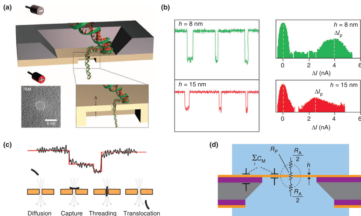
FIGURE 3 | (a) An illustration of a double-stranded DNA molecule passing through a solid-state nanopore. Inset, a TEM image of a silicon nitride nanopore. (b) Current signals from translocations through SiNx nanopores can be as large as several nanoamperes. (c) Nanopore current blockades are sensitive to the orientation and position of a translocating molecule. (d) Simplified electrical equivalent circuit of a solid-state nanopore, highlighting the access resistance R_A and the membrane capacitance C_M [(a) and (b): Reprinted with permission from Ref 35; (c) and (d): Reprinted with permission from Ref 51].
