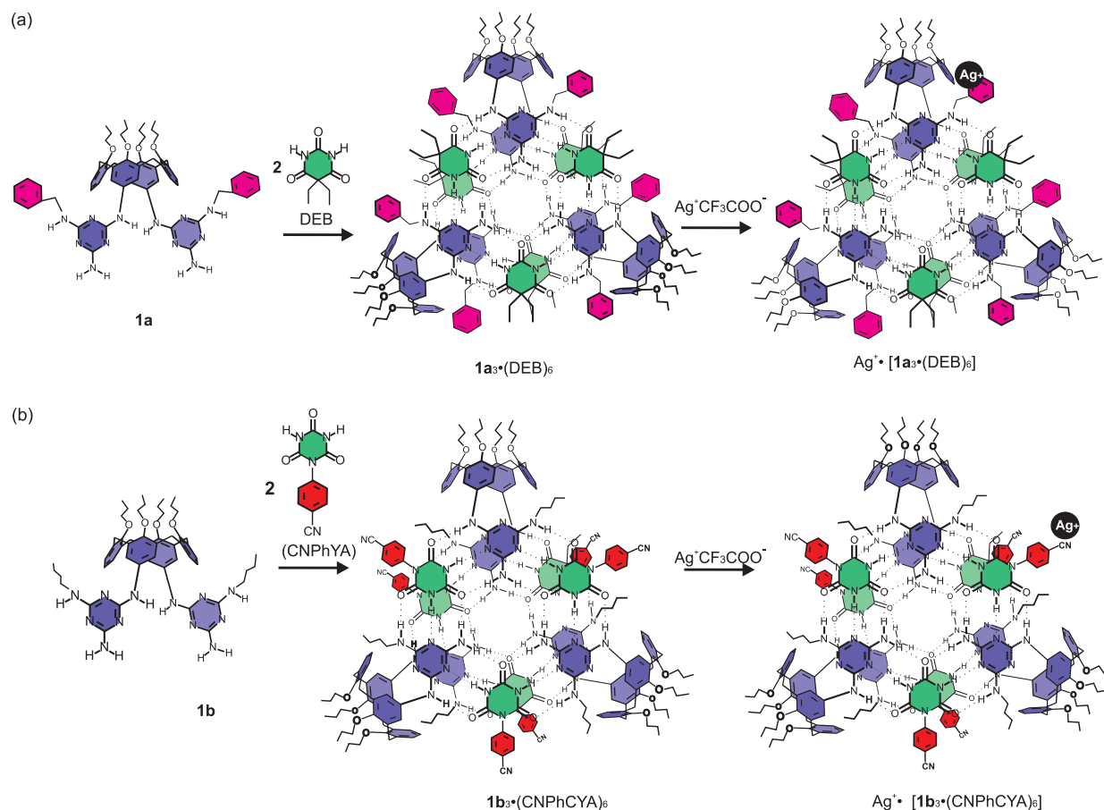
FIGURE 1 Synthesis of silver-functionalised double rosette assemblies \text{Ag}^+ \cdot [1a_3 \cdot (\text{DEB})_6] and \text{Ag}^+ \cdot [1b_3 \cdot (\text{CNPhYA})_6] .
