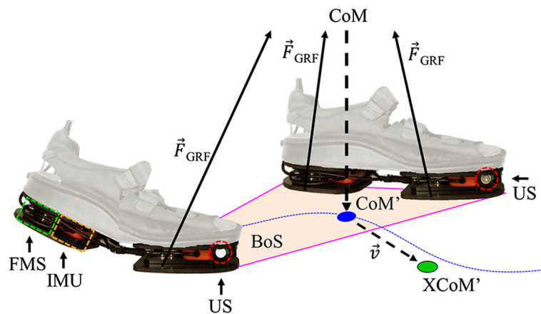
Fig. 1 Measurement setup. In this study Xsens ForceShoes™ were used, sandals with underneath one inertial measurement unit (IMU, dashed orange square ) and one force/moment (FMS, dashed green square ) sensor per heel or forefoot segment. Near the IMU in the forefeet an ultrasound transducer (US, dashed red circle ) was mounted in each shoe. Kinematic and kinetic data were used to estimate the position of the center of mass (CoM) relative to the position of both feet, the projection of the center of mass on the ground (CoM' - blue circle ) within the base of support (BoS) and the extrapolated CoM (XCoM' - green circle )
