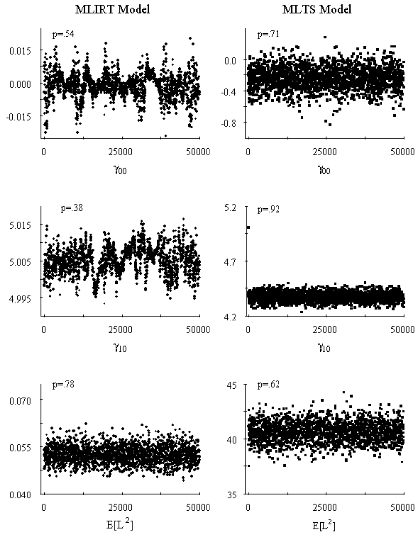
Figure 1. MCMC iterations of the model parameters and fit statistic corresponding to the MLIRT and the MLTS model. The p-values correspond to Geweke's MCMC convergence statistic.
