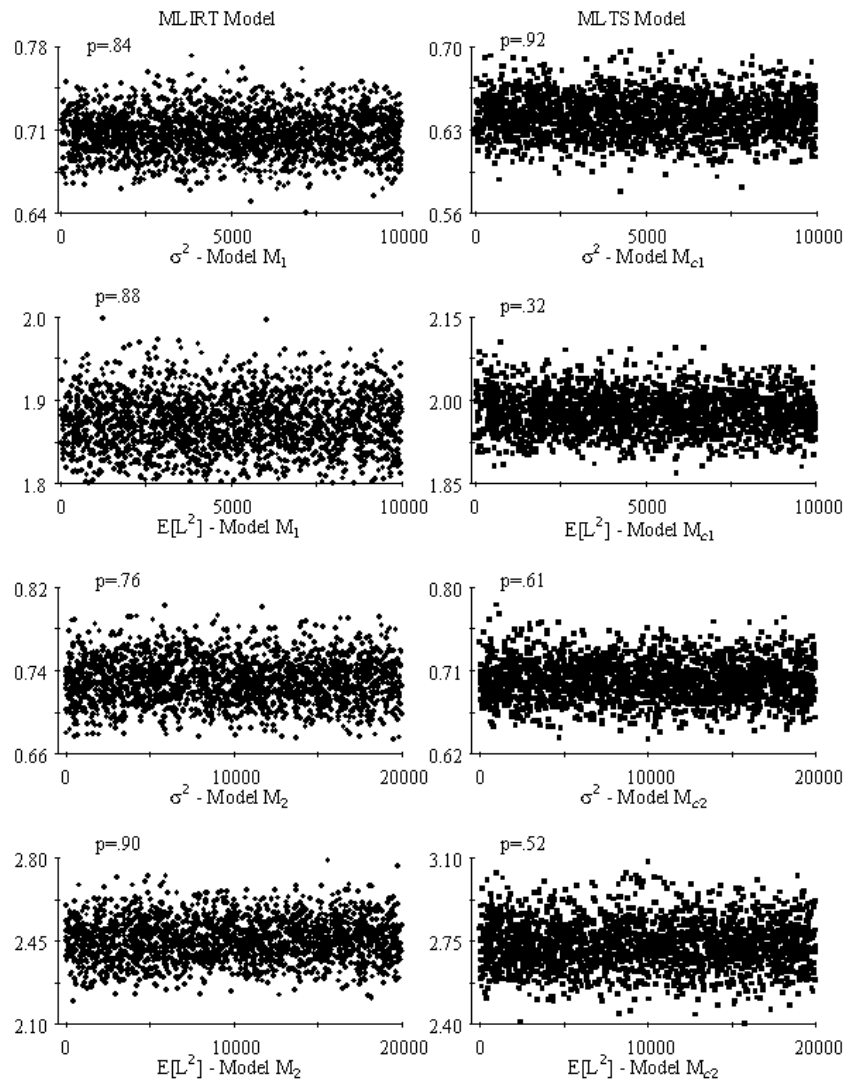
Figure 4. MCMC iterations of a variance parameter and the fit statistic corresponding to four different models. The p-values correspond to Geweke's MCMC convergence statistic.
