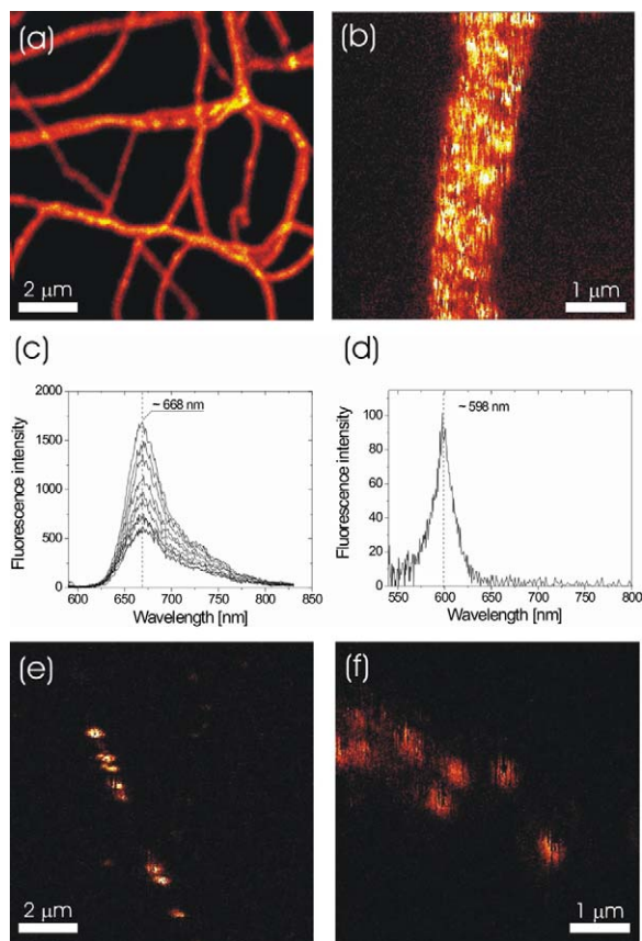
Fig. 2. Scanning confocal fluorescence images of (a) DiIC 1 (5) and (b) CdSe/ZnS quantum dots embedded in electrospun PEO fibers. The chromophores are distributed uniformly within and along the fibers, (c) Fluorescence emission spectra taken from individual fibers with embedded DiIC 1 (5) molecules, (d) emission spectrum of an individual QD embedded in a PEO fiber, and (e, f) single DiIC 1 (5) molecules and QDs along PMMA fibers. Characteristic blinking behavior is clearly visible and indicates that the fluorescence is coming from single light emitters.
