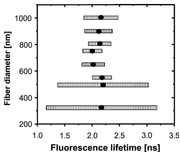
Fig. 4. Mean values of \tau_f distributions as a function of fiber diameter. The horizontal bars represent the widths of the \tau_f distributions. Significant broadening of the distributions for fiber diameters of 500 nm and below is clearly visible.
