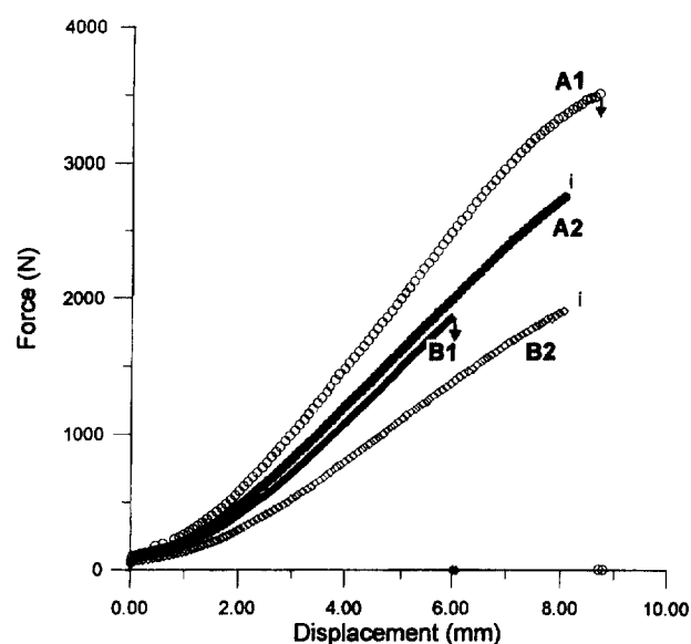
Fig. 1. Displacement versus applied force during deep drawing at 1210°C of several Y-TZP's with identical grain size (250 nm sample A and B; see Table 1). A1 and B1: displacement rate 0.6 mm min -1 ; A2 and B2: displacement rate: 0.3 mm min -1 .
