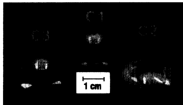
Fig. 5. Y-TZP samples with grain size of 125 nm after deformation tests; C3: deformed at 1160^\circ\text{C} with 0.3 \text{ mm min}^{-1} (height: 8 mm); C1: deformed at 1210^\circ\text{C} with 0.6 \text{ mm min}^{-1} (height: 10 mm); C2: deformed at 1150^\circ\text{C} with 0.6 \text{ mm min}^{-1} (height at fracture 4.3 mm).
