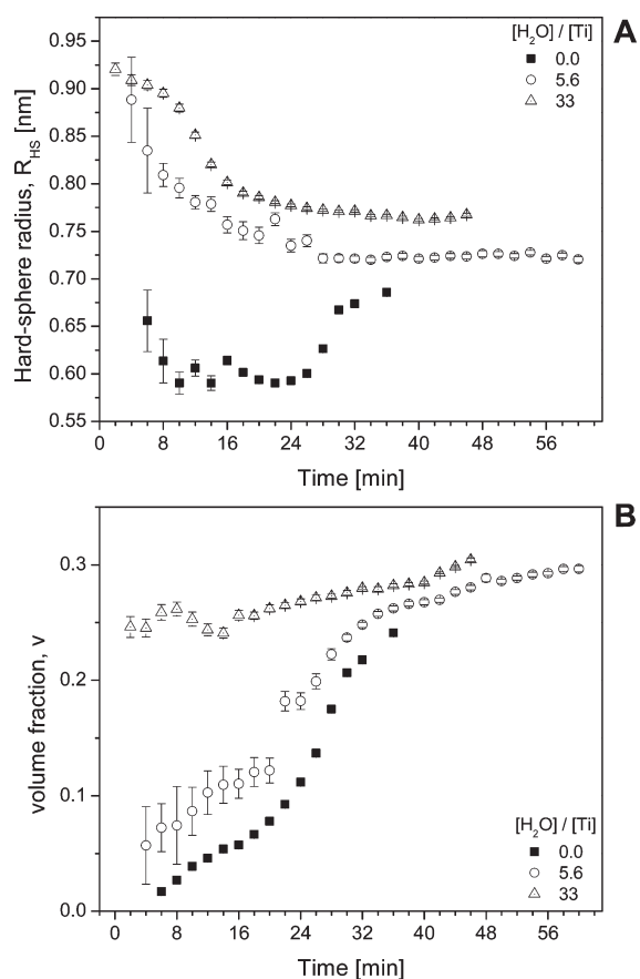
Figure 6. Fitted parameters from correlation structure factor S_C(q) : (a) hard-sphere radius 2R_{HS} . (b) volume fraction, v .
