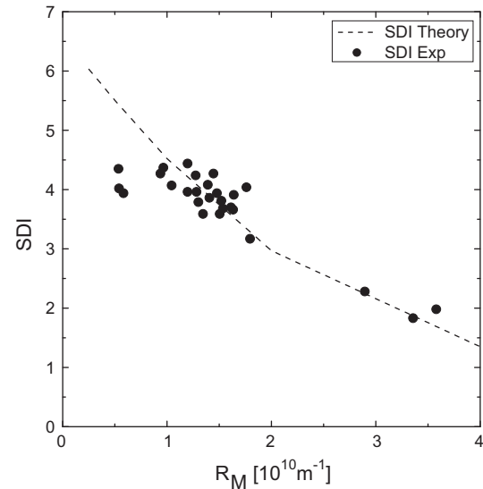
Fig. 5. SDI experimental and theoretical results for different membrane resistance materials and manufactures. The experiments carried out using particles concentration 4 ppm of AKP-15 under pressure 207 kPa.
