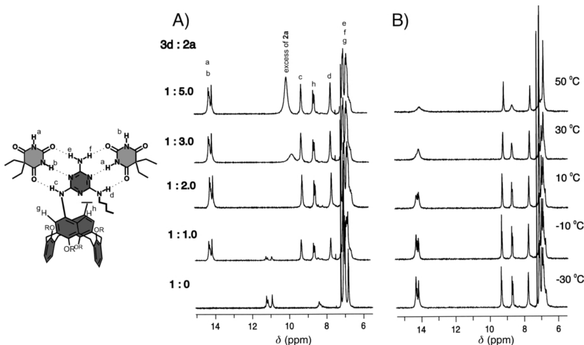
Fig. 6 A) ^1\text{H} NMR spectroscopic titration (400 MHz, \text{CDCl}_3 ) of 1,3-alternate calix[4]arene dimelamine 3d and barbituric acid 2a at -50\text{ }^\circ\text{C} , and B) partial variable temperature ^1\text{H} NMR spectra of double rosette assembly DR4 .
