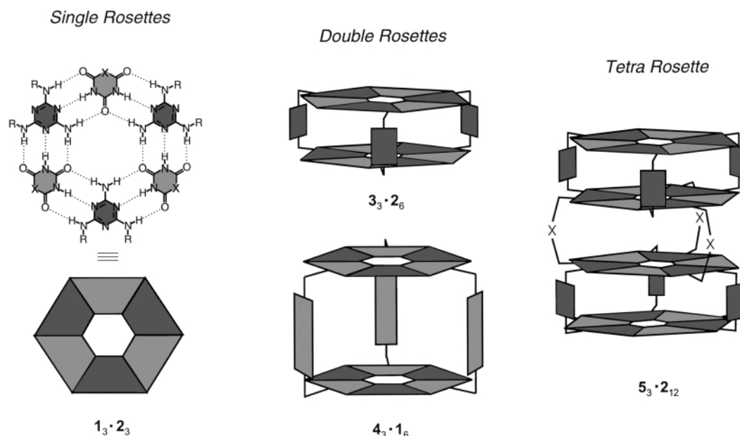
Fig. 1 Chemical structure and schematic representation of single rosette assembly 1 3 ·2 3 , double rosette assemblies 3 3 ·2 6 and 4 3 ·1 6 , and tetra-rosette assembly 5 3 ·2 12 .
