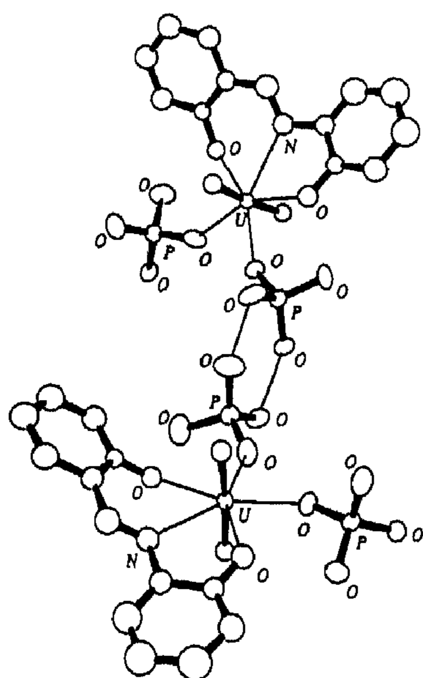
Figure 4. Crystal structure of the complex 19a \cdot 2H_2PO_4^- . The structure shown contains a crystallographic center of symmetry. Tetrabutylammonium fragments and solvent molecule are omitted for clarity.
