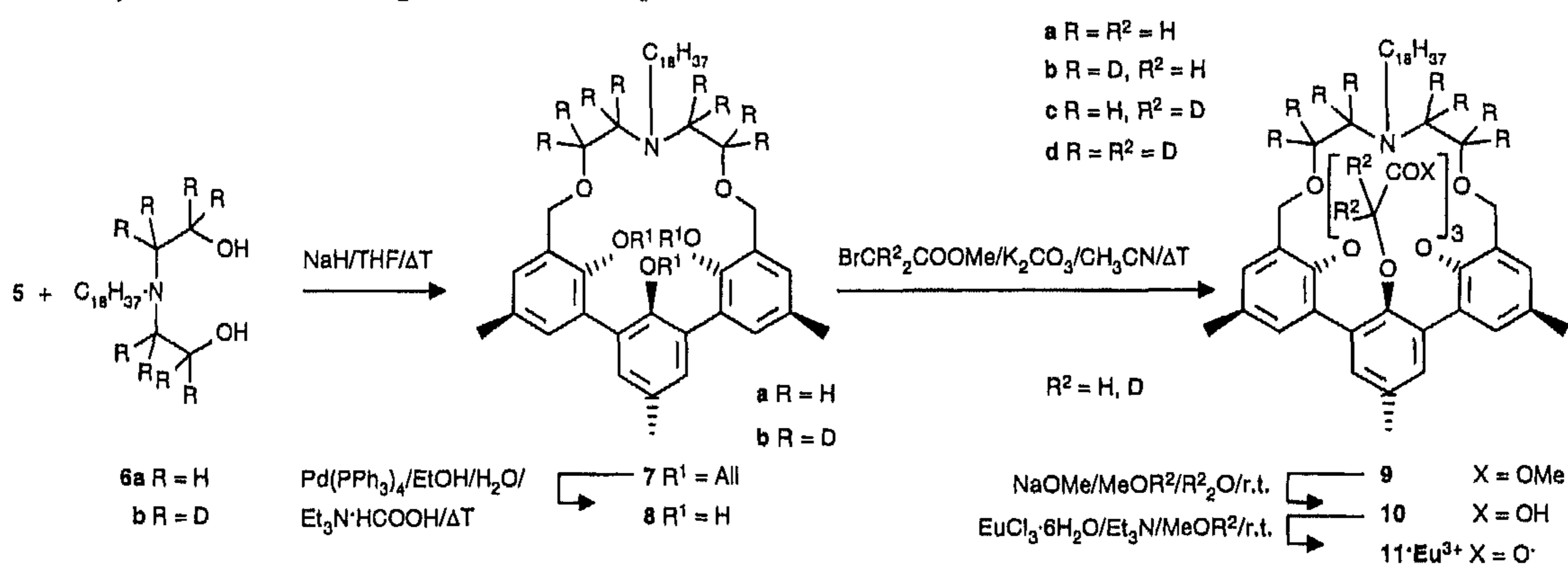
Scheme 2. Synthetic Route Leading to the Eu 3+ Complexes 11a–d·Eu 3+
