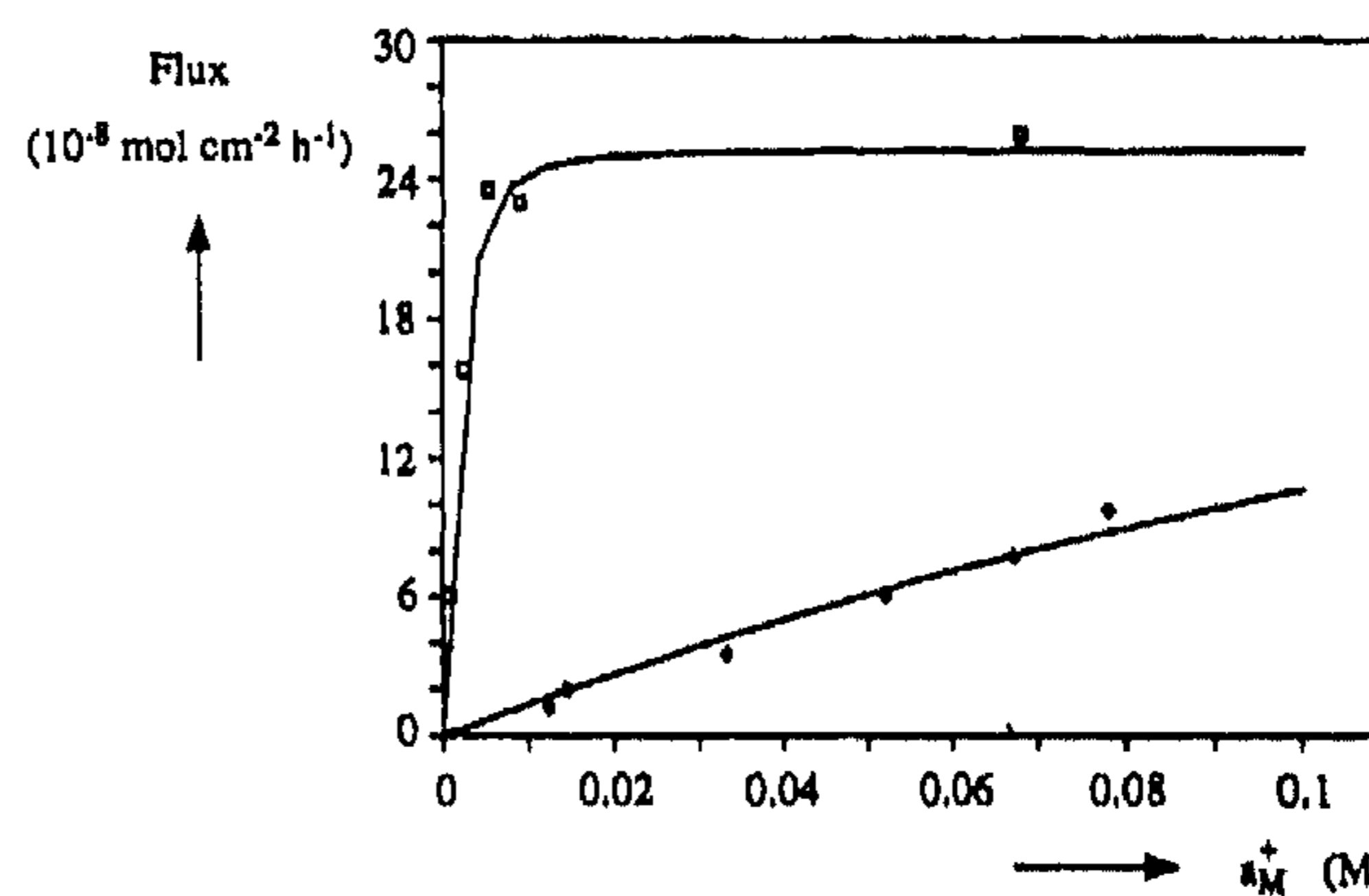
Figure 5. \text{KClO}_4 and \text{NaClO}_4 flux as a function of the salt activity in the source phase for valinomycin 6; [carrier] m 0 = 10^{-2} M, T = 298 K ( \diamond = \text{NaClO}_4 , \square = \text{KClO}_4 ). The lines drawn are calculated according to the model, the points are measured values.
