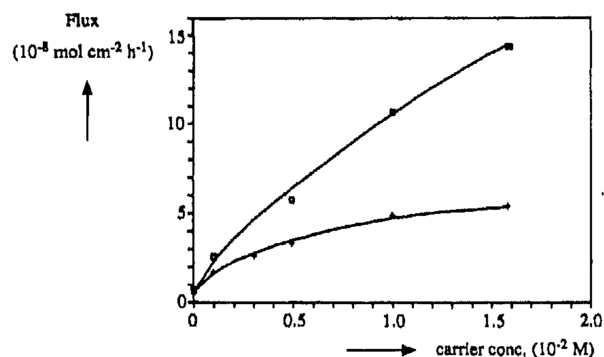
Figure 2. \text{KClO}_4 and \text{NaClO}_4 flux as a function of the calixcrown 5 concentration in NPOE; [alkali perchlorate] = 0.1 M, T = 298 K (+ = \text{NaClO}_4 , \square = \text{KClO}_4 ).
