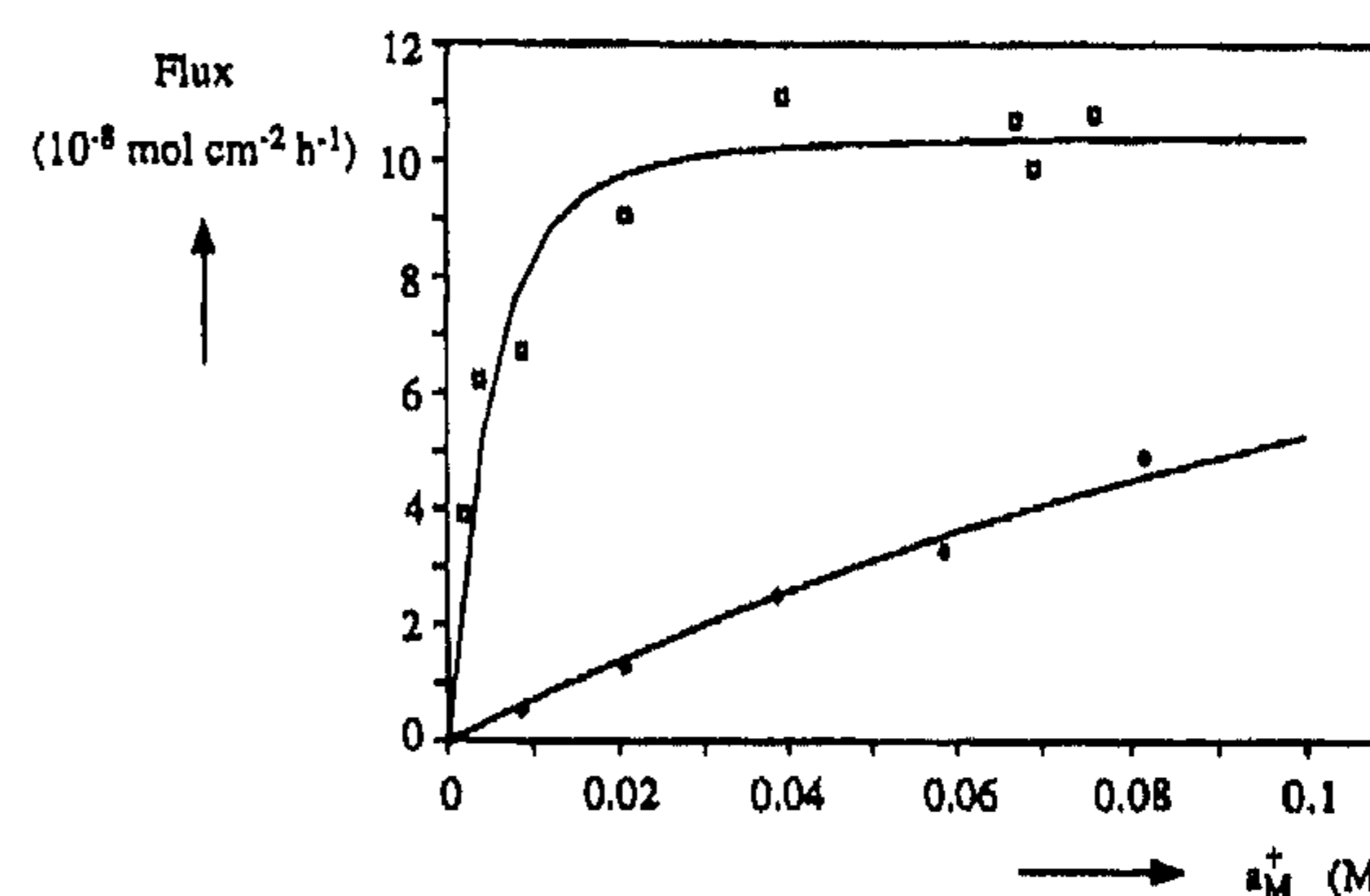
Figure 4. \text{KClO}_4 and \text{NaClO}_4 flux as a function of the salt activity in the source phase for calixcrown 5; [carrier] m 0 = 10^{-2} M, T = 298 K ( \diamond = \text{NaClO}_4 , \square = \text{KClO}_4 ). The lines drawn are calculated according to the model, the points are measured values.
