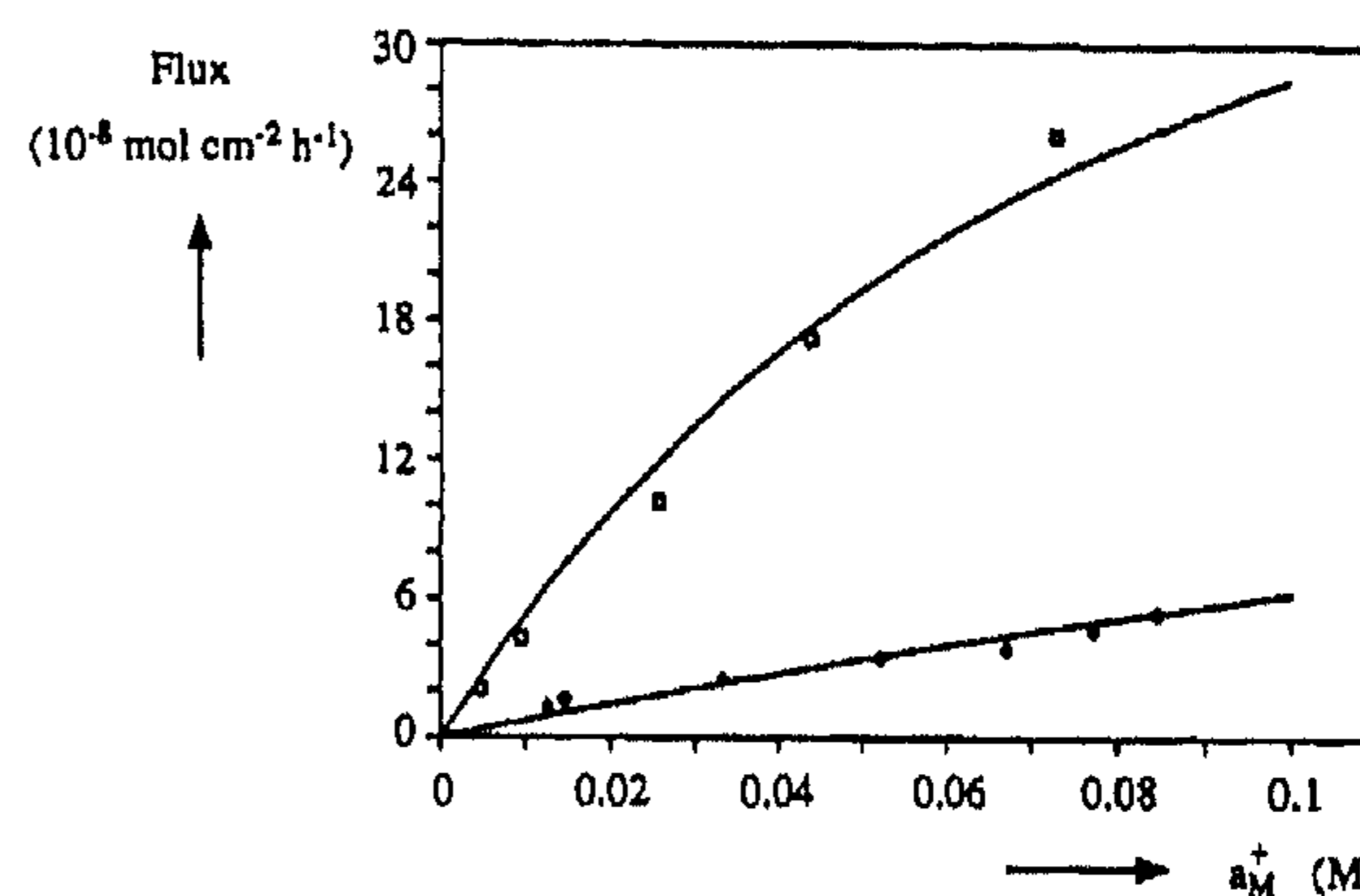
Figure 3. \text{KClO}_4 and \text{NaClO}_4 flux as a function of the salt activity in the source phase for dibenzo-18-crown-6 (1); [carrier] m 0 = 10^{-2} M, T = 298 K ( \diamond = \text{NaClO}_4 , \square = \text{KClO}_4 ). The lines drawn are calculated according to the model, the points are measured values.
