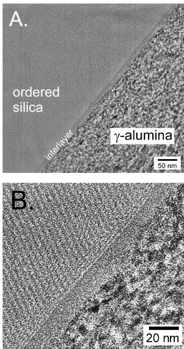
Fig. 3. (A) TEM image showing an ordered silica layer on a mesoporous \gamma -alumina layer with a structurally disordered silica-rich interface of 10–20 nm thickness; (B) enlarged TEM image showing ordering of silica layer parallel to the interlayer.
