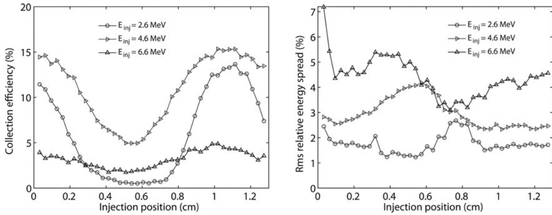
Fig. 7. The minimum RMS relative energy spread and collection efficiency of the accelerated bunches versus the injection position of the externally injected electron bunch. In this case, a_0 = 0.6 and \alpha = 6^\circ . The curves are shown for kinetic injection energies of 2.6, 4.6, and 6.6 MeV.
