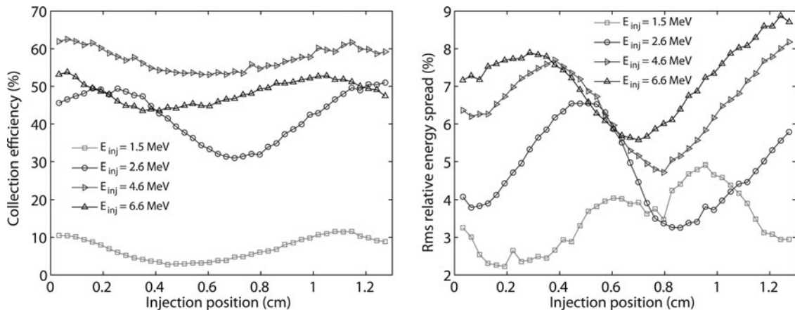
Fig. 8. The minimum RMS relative energy spread and collection efficiency of the accelerated bunches versus the injection position of the externally injected electron bunch. In this case, a_0 = 0.8 and \alpha = 2^\circ . The curves are shown for kinetic injection energies of 1.5, 2.6, 4.6, and 6.6 MeV.
