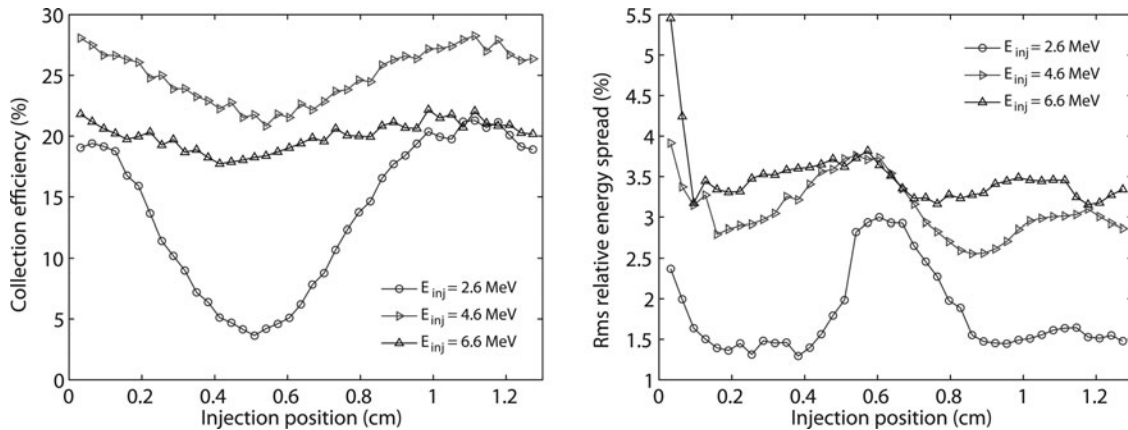
Fig. 6. The minimum RMS relative energy spread and collection efficiency of the accelerated bunches versus the injection position of the externally injected electron bunch. In this case, a_0 = 0.6 and \alpha = 4^\circ . The curves are shown for kinetic injection energies of 2.6, 4.6, and 6.6 MeV.
