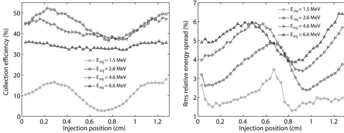
Fig. 9. The minimum RMS relative energy spread and collection efficiency of the accelerated bunches versus the injection position of the externally injected electron bunch. In this case, a_0 = 0.8 and \alpha = 4^\circ . The curves are shown for kinetic injection energies of 1.5, 2.6, 4.6, and 6.6 MeV.
