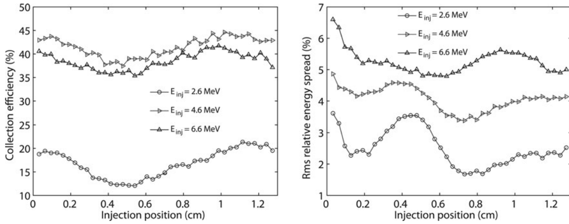
Fig. 5. The minimum RMS relative energy spread and collection efficiency of the accelerated bunches versus the injection position of the externally injected electron bunch. In this case, a_0 = 0.6 and \alpha = 2^\circ . The curves are shown for kinetic injection energies of 2.6, 4.6, and 6.6 MeV.
