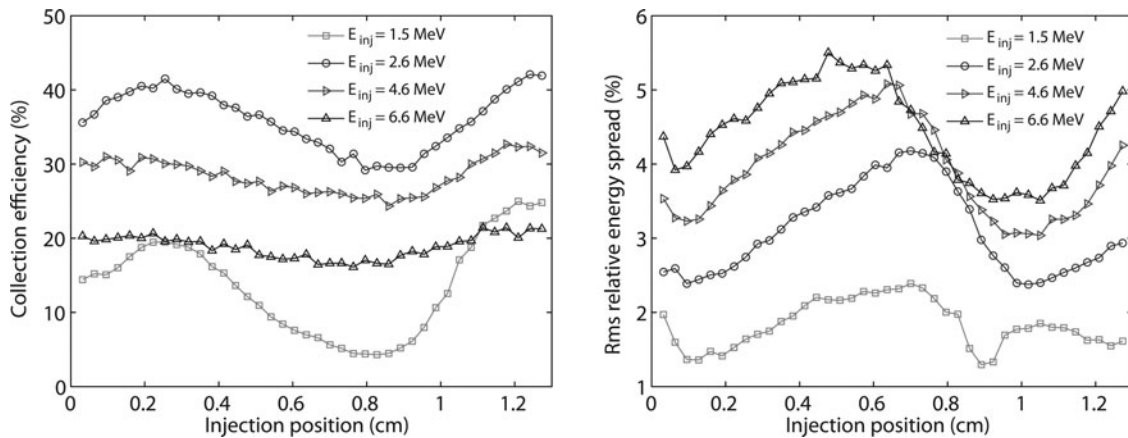
Fig. 10. The minimum RMS relative energy spread and collection efficiency of the accelerated bunches versus the injection position of the externally injected electron bunch. In this case, a_0 = 0.8 and \alpha = 6^\circ . The curves are shown for kinetic injection energies of 1.5, 2.6, 4.6, and 6.6 MeV.
