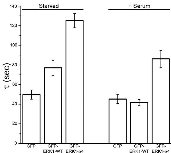
FIGURE 4. FRAP measurements with photobleaching of the entire nucleus to measure nuclear exchange. Comparison of GFP recovery after photobleaching the nucleus for free GFP, GFP-ERK1-WT, and GFP-ERK1- \Delta 4 . In both starved and stimulated state, WT recovery is faster than mutant.
