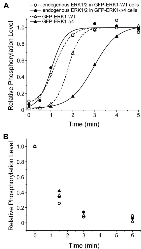
FIGURE 7. Phosphorylation kinetics were different for ERK1-WT and ERK1- \Delta 4 . A, plot of phosphorylation over time. Solid lines (cells transfected with mutant ERK) and hatched lines (cells transfected with wild type ERK) are sigmoidal fits to the data to determine the t_{1/2} values \pm 95% confidence interval (see text). Each trace was normalized to the fit maximum. B, relative phosphorylation levels of ERK1 in cells stimulated for 15 min and then treated with PD184359, blocking MEK activation and allowing the dephosphorylation of ERK.
