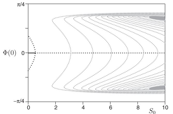
FIG. 8. Typical bifurcation diagram for the buckling induced instability, obtained from numerical integration of Eqs. (29) and (30). Solutions branches characterized by the angle at the bottom of the plate, \phi(0) , upon varying the buckling strengths S_0 . The values of T_0 = 0.25 and \theta_e = 2\pi/3 were kept fixed.
