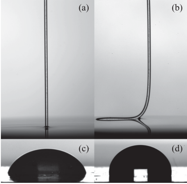
FIG. 1. (a), (b) Photographs of an elastomeric wire of radius R = 300 \mu\text{m} and density \rho = 1.02 \times 10^3 \text{ kg/m}^3 brought into contact with a mixture of ethanol and water. From (a) to (b), the contact angle is increased continuously by decreasing the concentration of ethyl alcohol. The wire exhibits a buckling instability above a critical contact angle. (c), (d) Independent determination of the contact angle, using drops of the same mixture on a plane substrate made of the same elastomer as in (a) and (b). On the left, the advancing contact angle is 60^\circ with a 50% volumic solution of ethyl alcohol in water. On the right, the advancing contact angle is 95^\circ with a 5% volumic solution of ethyl alcohol in water. In this figure we provide an illustrative example corresponding to an elastomeric wire, while in the rest of the paper we analyze a thin elastic plate—instability mechanisms are qualitatively similar for these two different systems.
