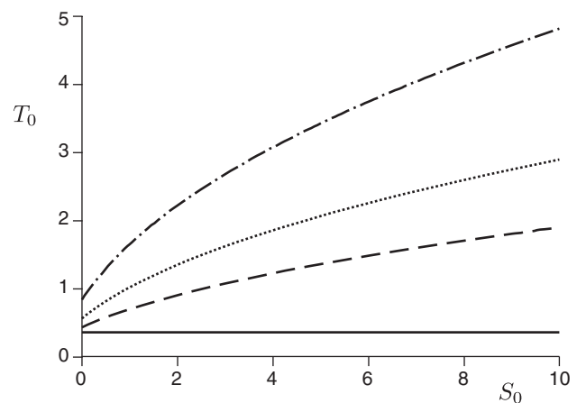
FIG. 5. The threshold of stability T_0 versus S_0 for different values of the contact angle \theta_e = \pi/6, \pi/4, \pi/3, \pi/2 . For \cos \theta_e > 0 , the bending threshold T_0 increases with S_0 since the vertical capillary force has a stabilizing effect. The limiting case \cos \theta_e = 0 has F_z = 0 , for which the bending threshold is independent of S_0 .
