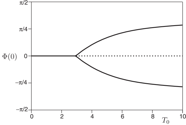
FIG. 6. Typical bifurcation diagram for bending induced instability, obtained from numerical integration of Eqs. (29) and (30). Solutions branches characterized by the angle at the bottom of the plate, \Phi(0) , upon varying the bending strength T_0 . The values of S_0 = 10.0 and \theta_e = \pi/4 were kept fixed.
