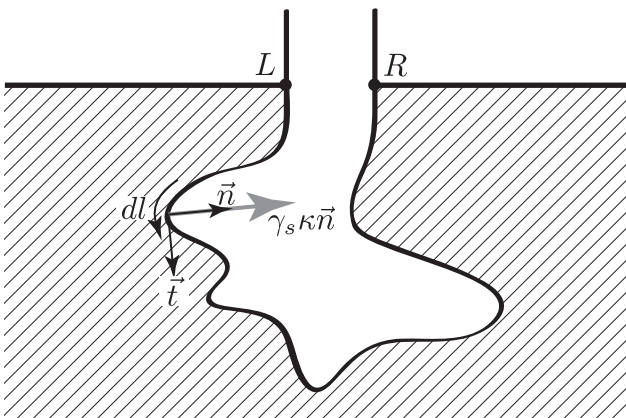
FIG. 13. Sketch of the quantities required to compute the Laplace pressure exerted on a solid of arbitrary shape. See text for details.
