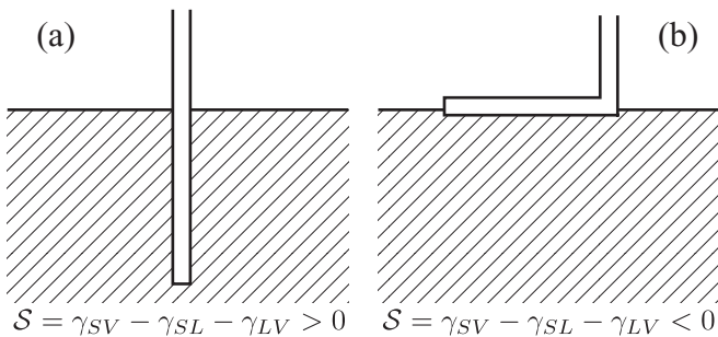
FIG. 2. Capillary energy of a partially immersed plate, in the absence of gravity and elasticity. (a) Two sides of the plate are immersed, representing an energy of 2\gamma_{SL} per immersed length. (b) When bending toward the surface, one of the sides is no longer wetted and part of the liquid-vapor interface is covered. The associated energy per length is \gamma_{SV} + \gamma_{SL} - \gamma_{LV} . The energy difference between (b) and (a) equals the spreading parameter S = \gamma_{SV} - \gamma_{SL} - \gamma_{LV} . For the partially wetting case S < 0 , so that state (b) is energetically more favorable than state (a).
