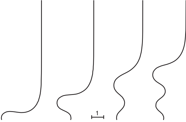
FIG. 9. Shapes of the plate with \Phi(0) = 0 for different buckling strengths S_0 . From left to right: S_0 = 2.689 , S_0 = 4.302 , S_0 = 5.636 , S_0 = 6.830 . The values of T_0 = 0.25 and \theta_e = 2\pi/3 are as in Fig. 8 and were kept fixed.
