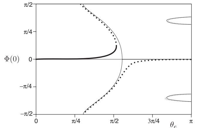
FIG. 12. Effect on hysteresis on the bifurcation diagram, \Phi(0) versus \theta_e , in the case H/\mathcal{H} = 1.71 and \ell_{EG}/\ell_\gamma = 250 . \Delta\theta = 0.1 (thick lines) is compared to the case without hysteresis (thin line). The hysteresis allows for stable solutions of nonzero amplitude \Phi(0) .
