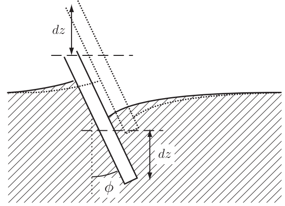
FIG. 4. The resultant vertical force on the plate can be obtained from the change in surface free energies due to a virtual displacement dz . See text for details.
