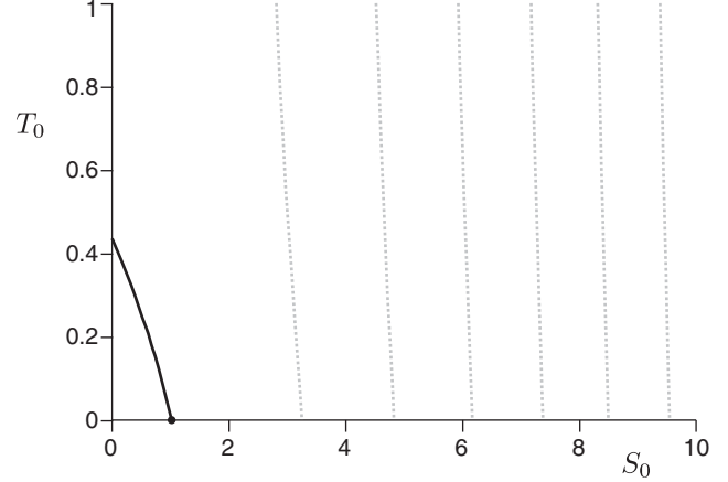
FIG. 7. The threshold of stability T_0 versus S_0 for \theta_e = 2\pi/3 . The vertical force F_z now compresses the wire and leads to buckling, even in the absence of bending ( T_0 = 0 ). Similar to the classical buckling instability, the higher order branches correspond to all extrema of the Airy function.
