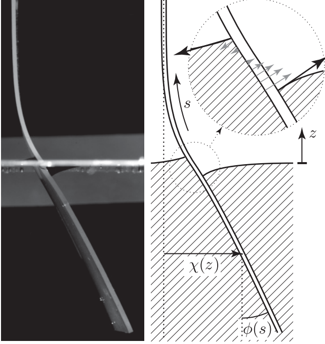
FIG. 3. Left: Photograph of an elastomeric plate partially bent by capillary forces. We show that such bending to a stable, finite angle is only possible due to contact angle hysteresis. The plate thickness is H = 0.8 mm, its Young modulus is E = 66 kPa, and its density is 1.02 \times 10^3 kg/m 3 . As not particularly clean tap water is used, the surface tension is around \gamma = 0.05 N/m. Right: Definitions of the vertical coordinate z and curvilinear coordinate s . The deformation of the plate is characterized by the deflection \chi(z) or local angle \phi(s) . The characteristic curvature of the plate is \ell_\chi^{-1} . Inset: sketch of the resultant capillary forces in the meniscus region. At the contact lines there are pulling forces along the liquid-vapor interface of magnitude \gamma . In addition, the hydrostatic pressure pulls or pushes on the plate depending on the level with respect to bath. The scale of the meniscus is \ell_\gamma .
