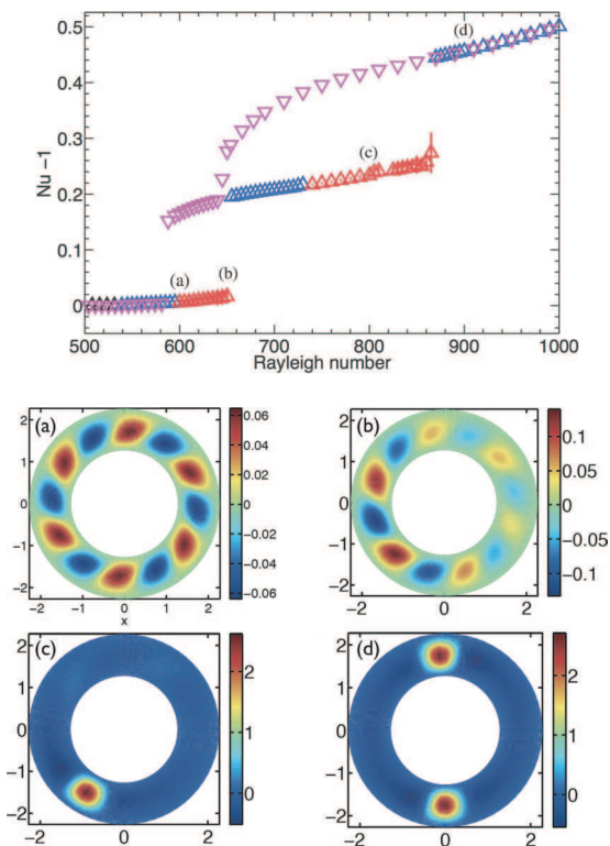
Fig. 5: (Color online) Numerical results for the dimensionless convective current, Nu - 1 , at \alpha = 0.56 , \mathcal{P} = 75.8 and Re = 0.231 . In comparison with fig. 2c for which Re = 0.124 , this larger shear produces more bifurcations over a similar range of the dimensionless control parameter. The spatial patterns of the perturbed stream function shown below are marked by letters in the upper plot. (a) Oscillatory convection at Re = 600 at t = 30\tau_q . (b) Undulating convection at a mode-changing bifurcation at Re = 650 at t = 30\tau_q . (c) Oscillatory and localized convection, consisting of a single vortex at Re = 800 at t = 20\tau_q . (d) Non-oscillatory, traveling localized convection at Re = 900 at t = 20\tau_q .
