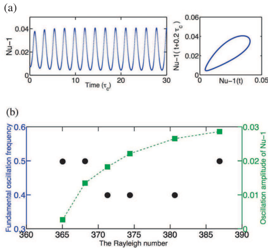
Fig. 3: (Color online) Numerical data for the oscillatory convective current Nu-1 for \alpha=0.56 , \mathcal{P}=75.8 , and \mathcal{R}e=0.124 : (a) the time-series data for \mathcal{R}=371.3 , together with the corresponding phase space trajectory, reconstructed using a time-delay method; (b) the fundamental frequencies ( \bullet ) and the oscillation amplitudes ( \blacksquare ) of Nu-1 as a function of \mathcal{R} .
