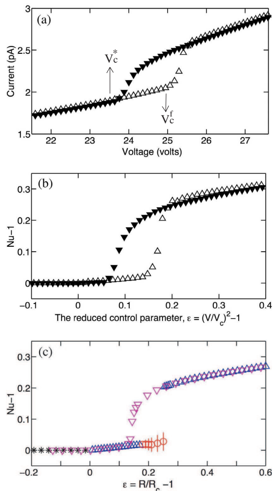
Fig. 2: (Color online) (a) Experimental raw current-voltage data from ref. [14] for \alpha = 0.56 , \mathcal{P} = 76 , and \mathcal{R}e = 0.124 . The open (filled) triangles are for increasing (decreasing) voltage. (b) The corresponding measured dimensionless convective current, Nu - 1 , vs. dimensionless control parameter \epsilon = (V/V_c)^2 - 1 , extracted from the data in (a). (c) Simulation results for Nu - 1 for the same parameters as in the previous experimental figure. The film undergoes a sequence of bifurcations as \mathcal{R} is slowly increased and then decreased ( \nabla ). The sequence of flow regimes are conduction (*), steady rotating convection ( \Delta ), and oscillatory rotating convection ( \circ ), with the vertical bars showing the amplitude of oscillation. A large hysteretic bifurcation is located at the jump in the dimensionless current that signals changes in the structure of the azimuthal Fourier modes.
