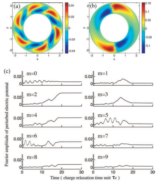
Fig. 4: (Color online) The spatial patterns of the electric potential perturbation, ( i.e. the total potential minus the conduction profile) at \mathcal{R}=388.0 and \mathcal{R}e=0.124 , as in fig. 2c. (a) Initially, there are six oscillatory traveling vortex pairs. (b) After 30\tau_q , there are two non-oscillatory traveling vortices. (c) Time series of the Fourier amplitudes of the perturbed electric potential at midradius, showing the mode evolution during the transition.
