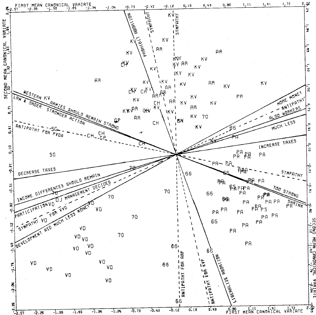
Figure 6. The MPs projected in the mean canonical space (numerical solution). The individuals are labelled by their party membership. The lines are the directions of the optimally scaled variables.
