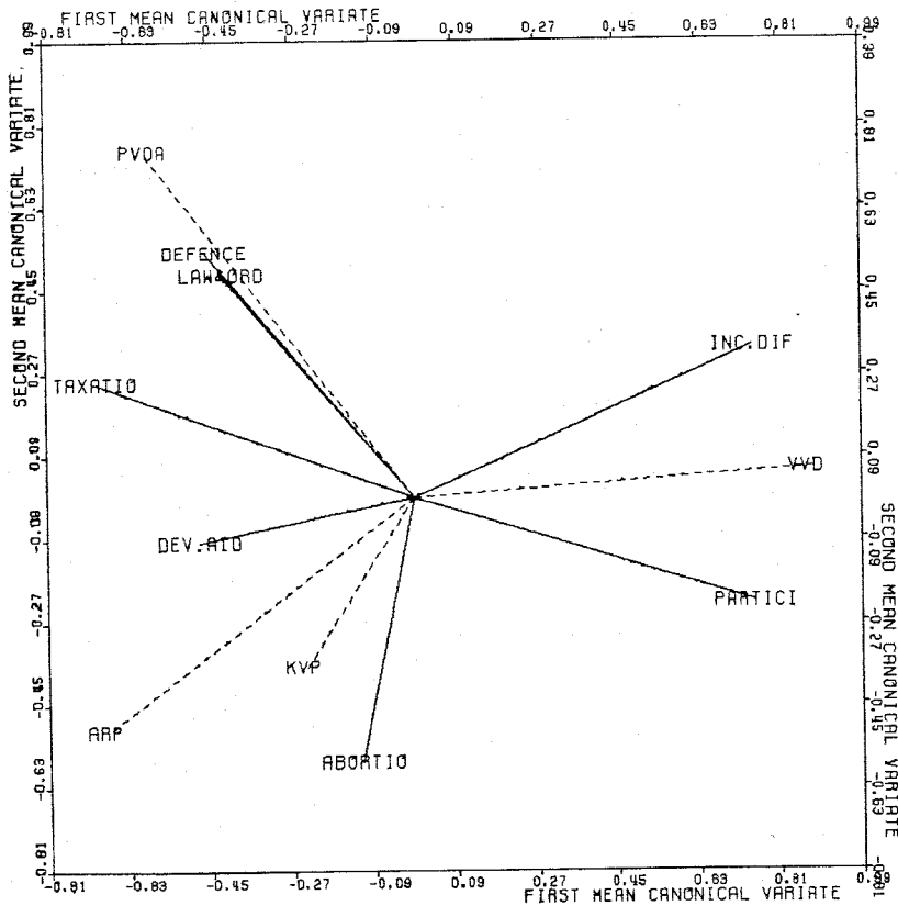
Figure 3. Component loadings: the projections of the optimally scaled variables in the mean canonical space (ordinal solution).
