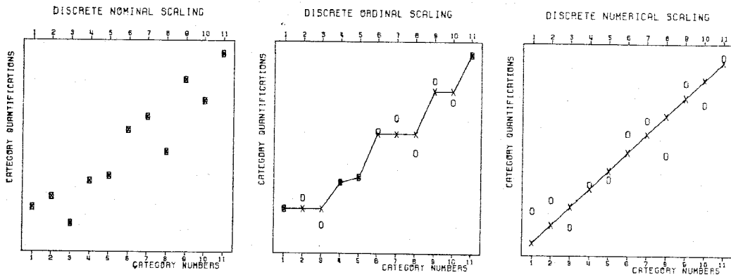
Figure 2. Different types of scaling. (o) category means ( \hat{q}_j ), \times regressed category means ( \tilde{q}_j ).
