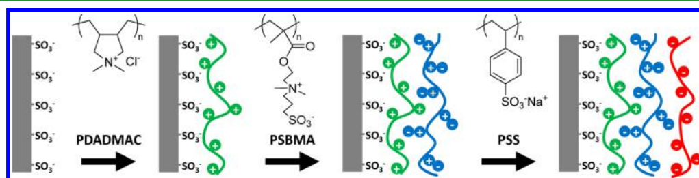
Figure 2. Schematic representation of the coating of a charged hollow fiber membrane with a trilayer of PDADMAC (+), PSBMA (z), and PSS (-) on a charged hollow fiber membrane.
