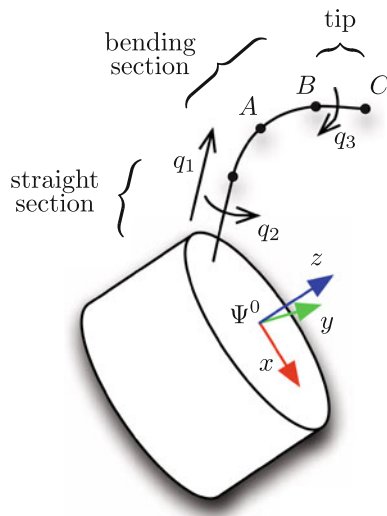
Fig. 2 The endoscopic instrument has three degrees of freedom: translation q_1 , rotation q_2 , and bending q_3 . Points A and B are located midway and at the end of the bendable section, respectively. Point C is located at the tip. Frame \Psi^0 denotes the camera frame of the endoscopic camera
