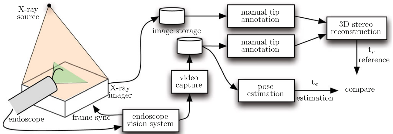
Fig. 6 The estimator was evaluated using an X-ray imaging setup. Images from the endoscopic camera and the X-ray imager were synchronously acquired and stored. In both the X-ray images and the endoscopic images, the tip position was manually annotated. From these positions,
