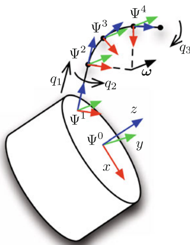
Fig. 13 Five frames are defined: frame \Psi^0 and \Psi^1 are fixed to the endoscope, while frame \Psi^2 , \Psi^3 and \Psi^4 are fixed along the instrument. q_1 , q_2 , and q_3 denote the three DOFs: insertion, rotation, and bending, respectively
