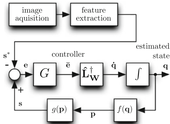
Fig. 4 Marker-less state estimation: For a given state q , the kinematic model f and camera model g are used to compute the expected positions of the feature points in the image space, denoted s . These are compared to s^* , which are the positions of the feature points in the endoscopic image, as determined by the feature extraction algorithm. The difference s - s^* , denoted e , is input to the controller, which computes the state change \dot{q} to bring the model closer to the observed instrument
