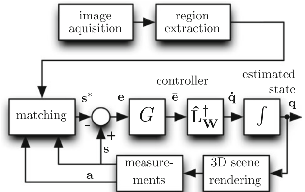
Fig. 5 Marker-based state estimation: The structure of the estimator is similar to the marker-less method, but the main difference is the extra matching step, in which the regions that are extracted from the endoscopic image are matched to the markers. For a given state q , a 3D rendering of the scene is created. From this scene, the centroids (denoted s ) and areas (denoted a ) of the rendered markers are computed. s is compared to s^* , which are the centroids of the markers in the endoscopic image. The difference s - s^* , denoted e , is input to the controller, which computes the state change \dot{q} to bring the model closer to the observed instrument
