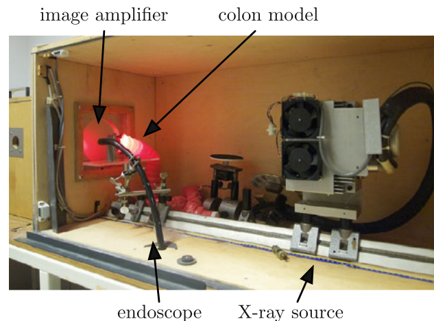
Fig. 8 A custom-built X-ray imaging setup was used for the experiment. The X-ray source generates the X-rays which are captured by the image amplifier. The images are digitized by a digital camera (not visible in the image). The endoscope is positioned inside a colon model during the experiment
