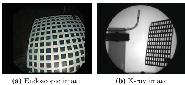
Fig. 9 The stereo rig composed of a the endoscope camera and b the X-ray imager is calibrated by imaging a reference object using both image modalities. In (a) , it can be observed that severe barrel distortion is present in the endoscopic images
