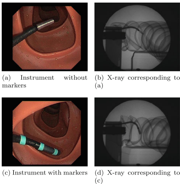
Fig. 10 During the experiment, the instrument was manually operated while the endoscope was inside the colon model. A top view of the scene was simultaneously imaged using an X-ray imager. In (a) and (b) , endoscopic and X-ray images of the experiment without markers are shown. In (c) and (d) images of the experiment with markers are shown
