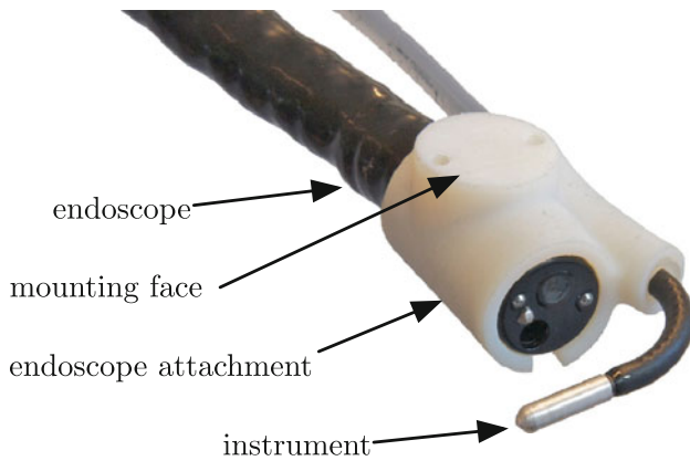
Fig. 7 An endoscope attachment was designed to let the endoscopic instrument emerge near the endoscopic camera, similar to the Anubis endoscope. The attachment also has a mounting face, which enables the endoscope to be fixed inside the X-ray imaging setup
