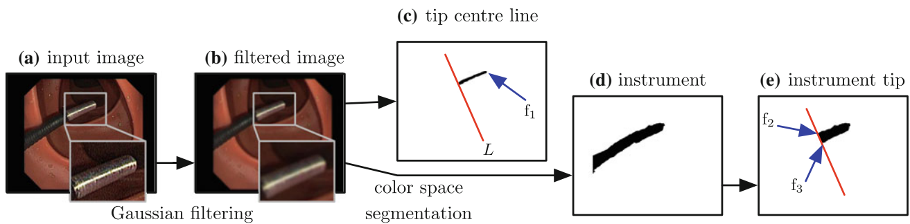
Fig. 3 Feature detection for the marker-less method: The input image (a) is filtered using a Gaussian filter kernel in order to remove noise. This results in image (b). This image is color-space-segmented twice using different parameters, resulting in the tip centerline (c) and the instrument (d) regions. From the tip centerline , the tip position is found,
