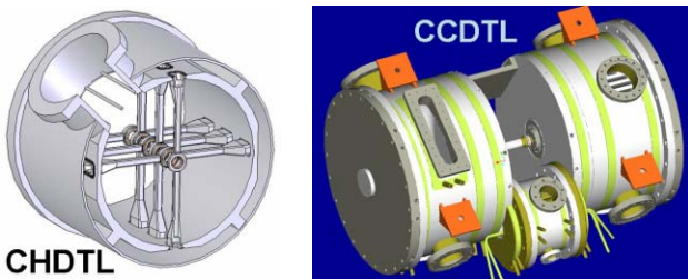
Figure 7: Drift Tube Linac designs
