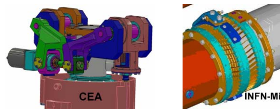
Figure 4: Design of two piezo-electric tuner prototypes
