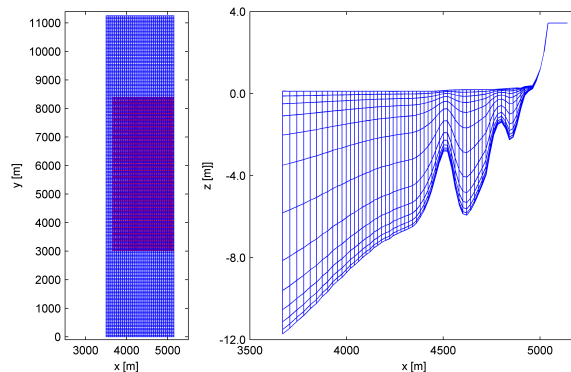
Figure 3. Plan view of FLOW (red) and WAVE (blue) grids (left) and side view of FLOW grid (right).
